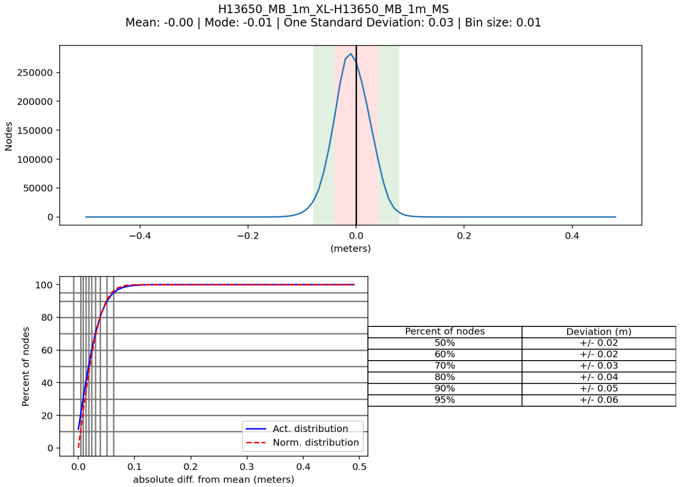
Figure 4: H13650 Crossline Difference
