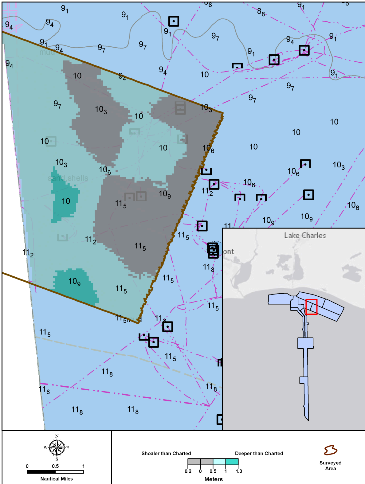
Figure 11: Depth Difference Between H13650 and US4LA14M
