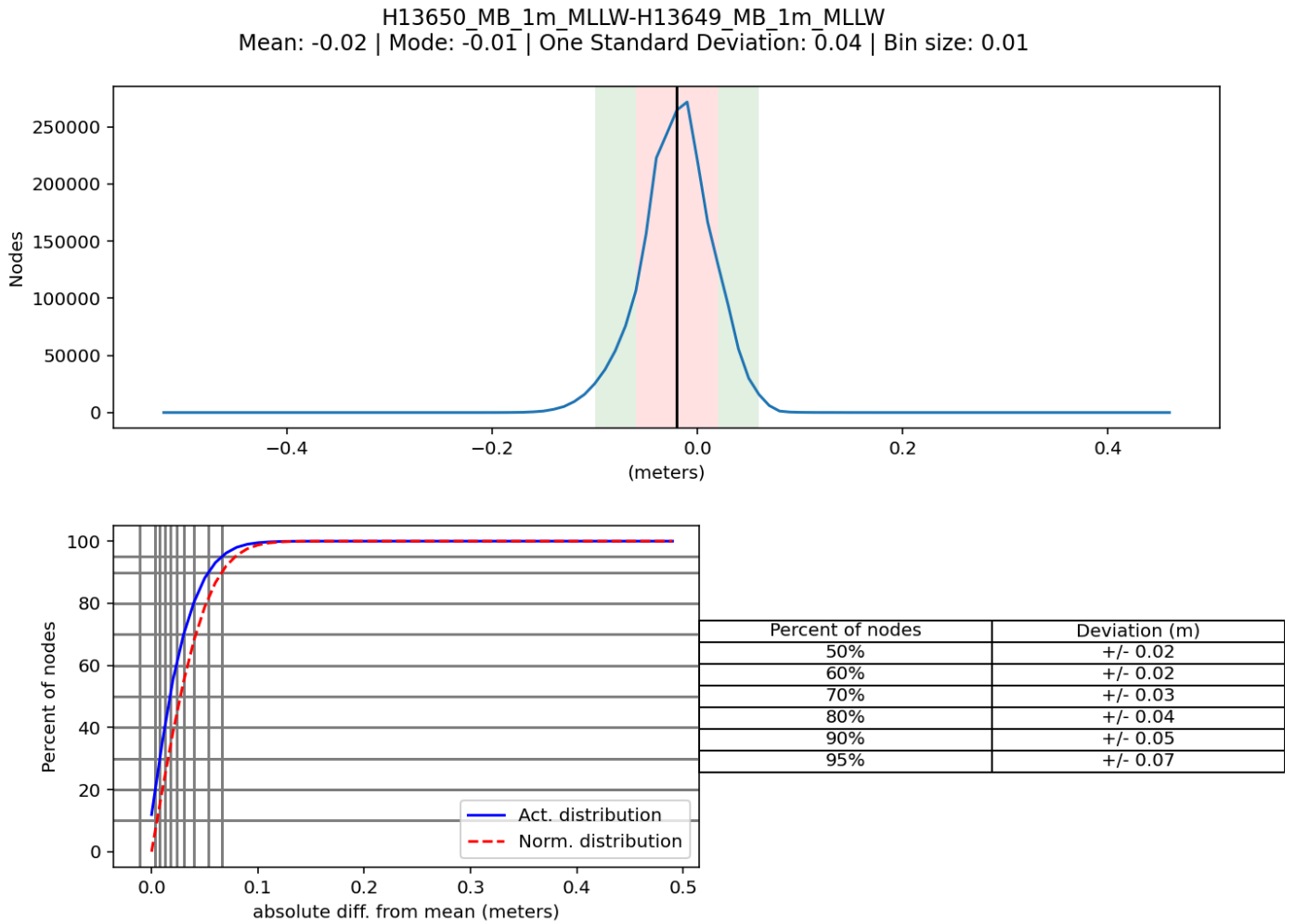
Figure 9: Distribution Summary Plot of Survey H13650 1-meter vs. H13649 1-meter
