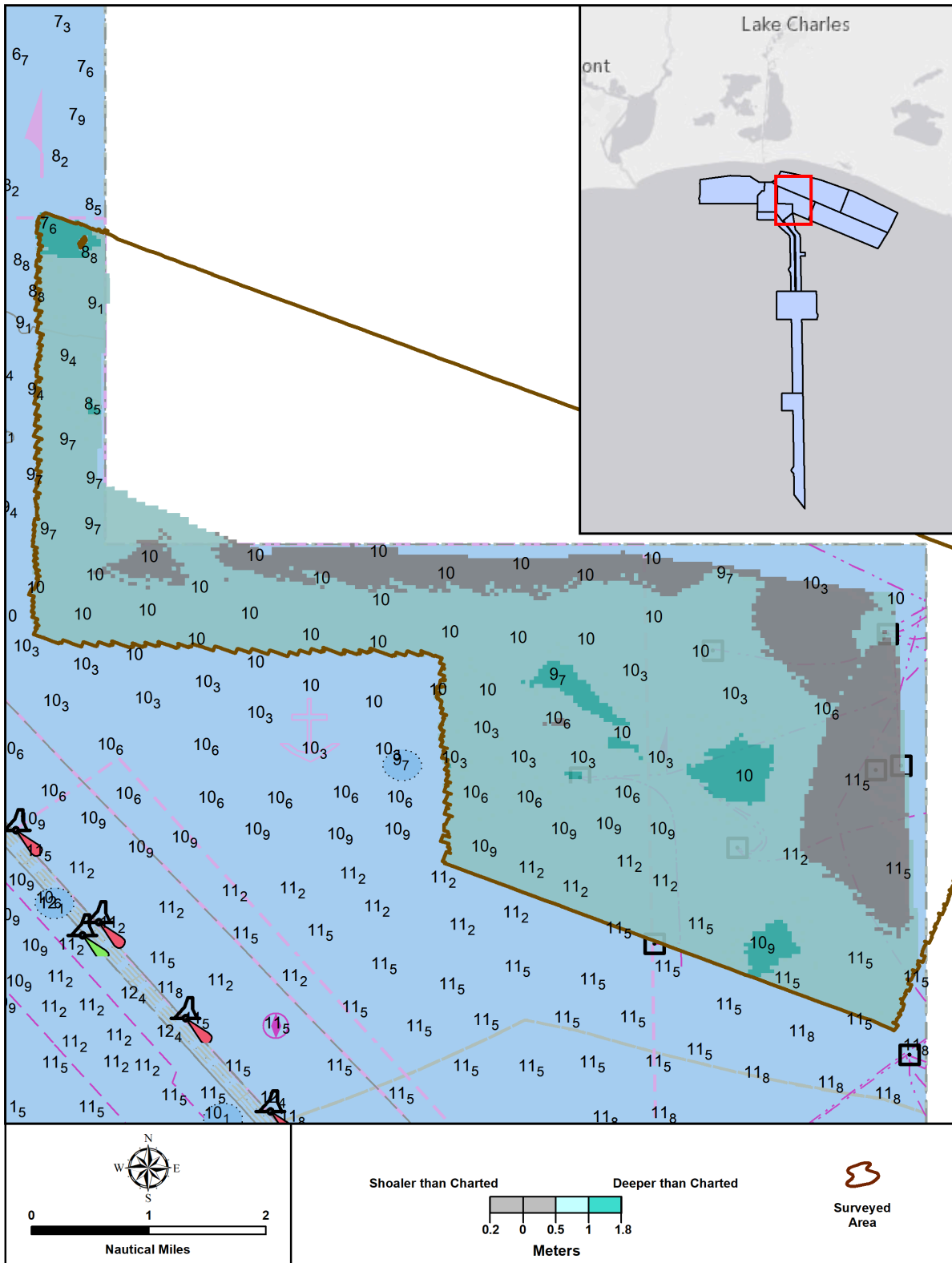
Figure 13: Depth Difference Between H13650 and US5LA16M
