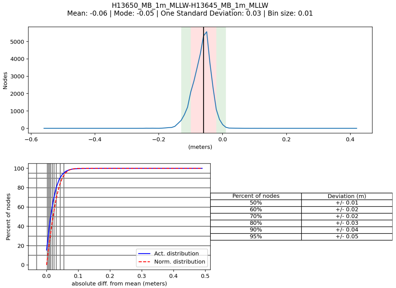
Figure 8: Distribution Summary Plot of Survey H13650 1-meter vs. H13645 50-centimeter
