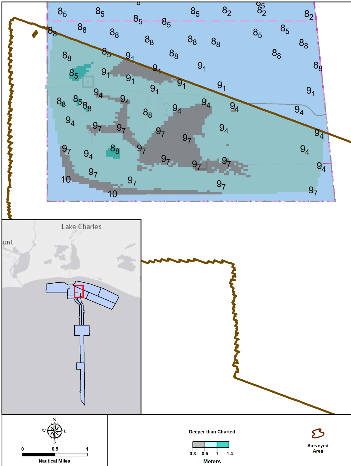
Figure 12: Depth Difference Between H13650 and US5LA11M
