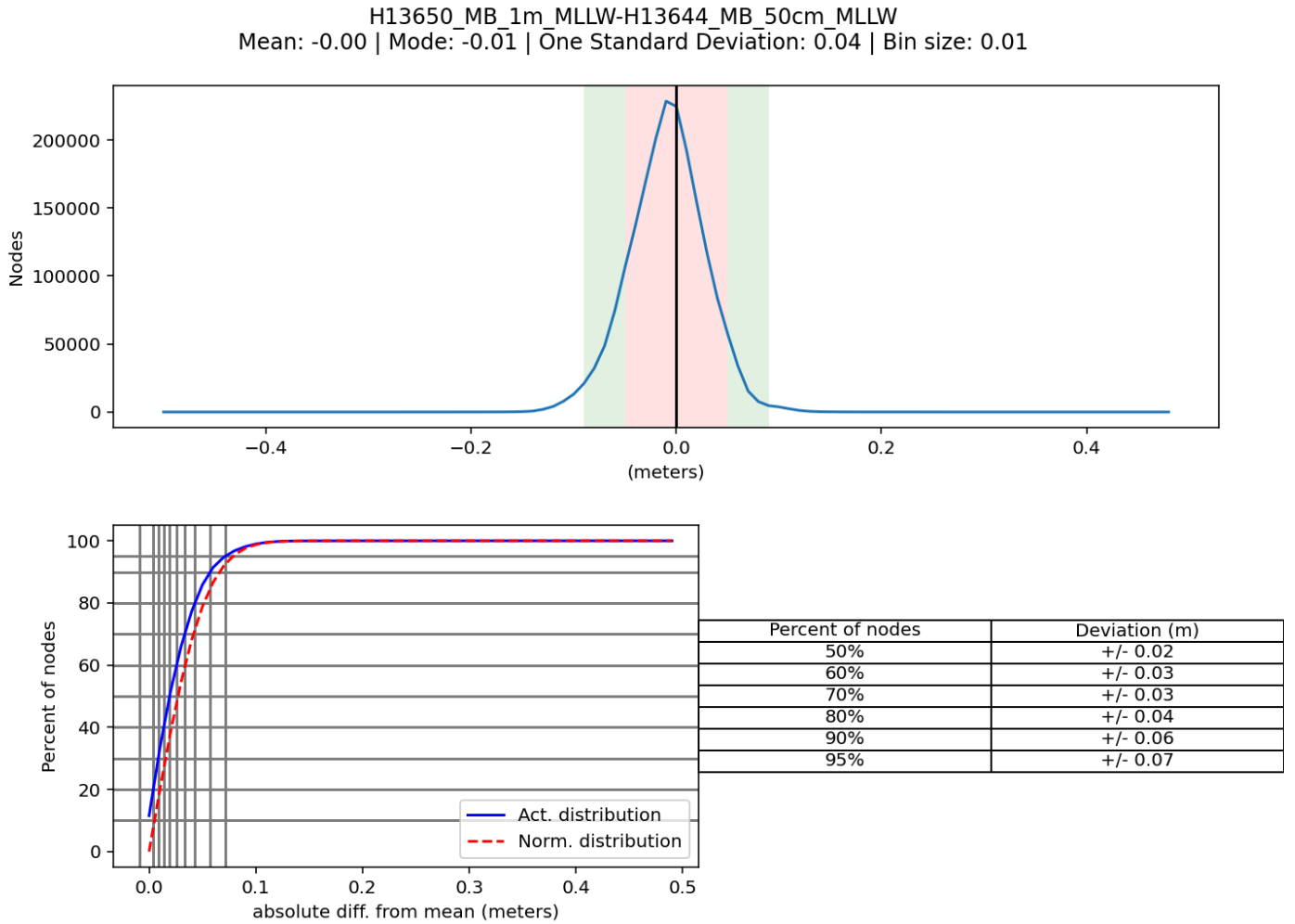
Figure 7: Distribution Summary Plot of Survey H13650 1-meter vs. H13644 50-centimeter
