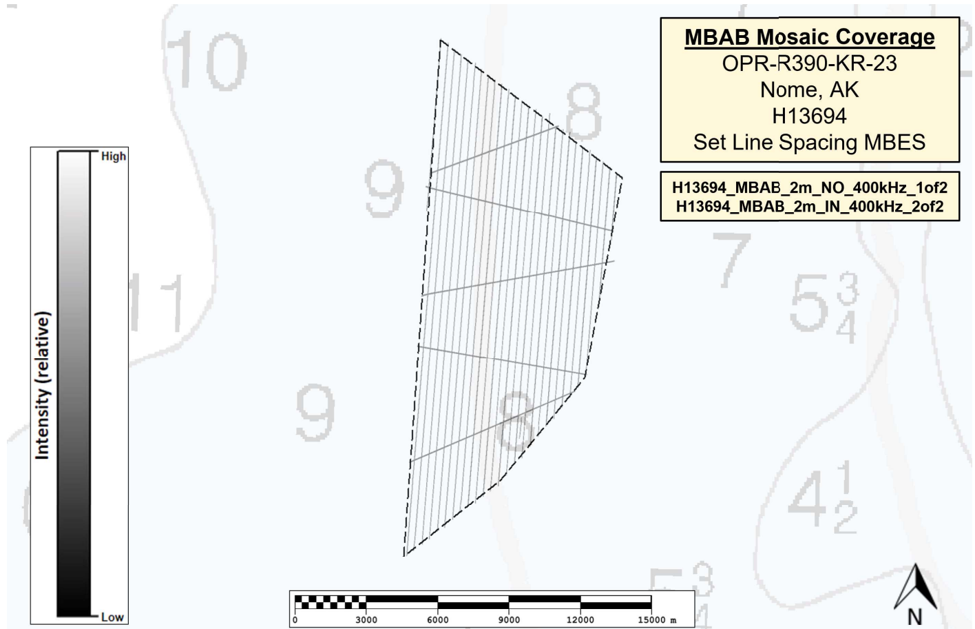
Figure 9: H13694 Finalized 2m MBAB Mosaic Coverage
