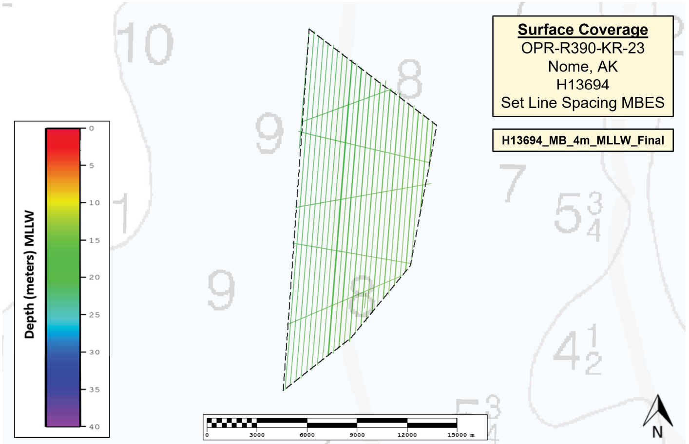
Figure 8: H13694 Finalized 4m CUBE weighted Dynamic Surface Coverage
