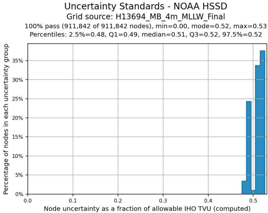
Figure 5: H13694 Finalized 4m MBES TVU Statistics
