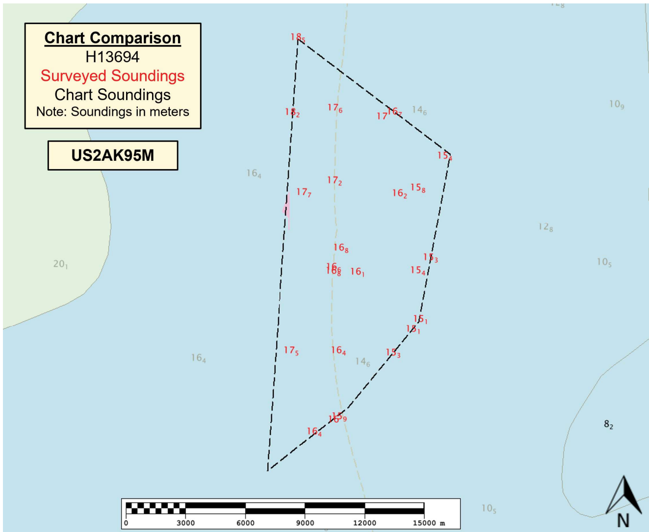
Figure 10: Generated Soundings used for Chart Comparison (US2AK95M)
