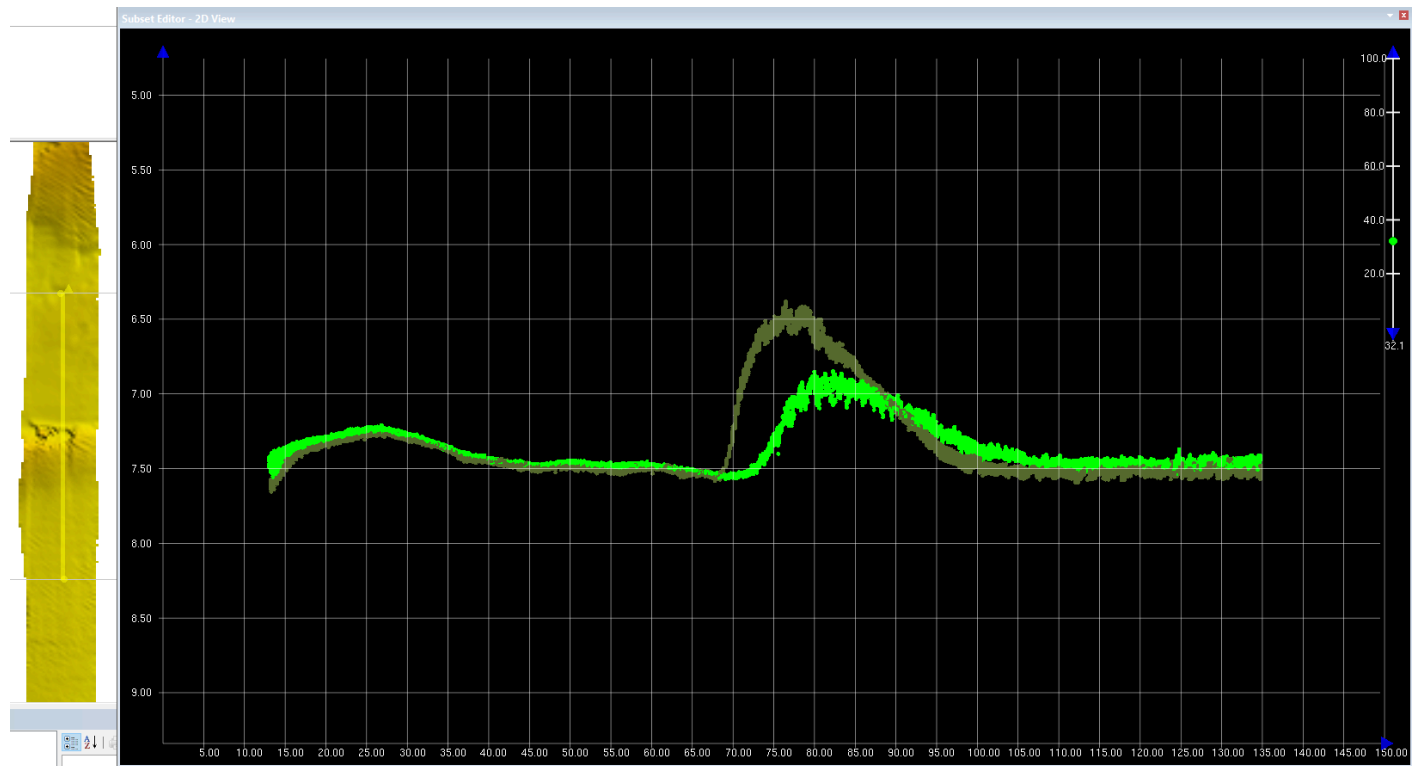
Figure 8: Example of bottom change on this survey viewed in CARIS HIPS subset. Dark green line (ASV, line 1756) was run on JD224, 59 days after the green line (Arctic Seal, 0293) run on JD165. This results in about 0.75 m of vertical change.
