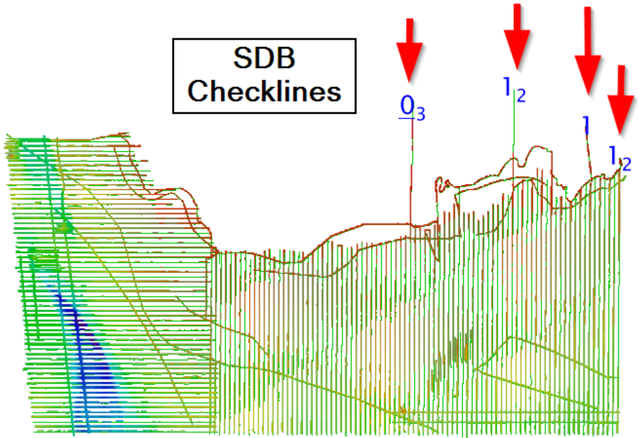
Figure 2: Image showing the relative location of SDB checklines. The least depth achieved on each checkline is shown in meters.
