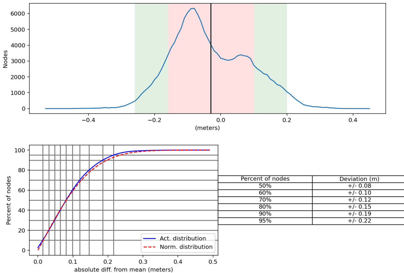
H13717 ASV versus Arctic Seal Depth Comparison Mean: -0.03 | Mode: -0.08 | One Standard Deviation: 0.12 | Bin size: 0.01
