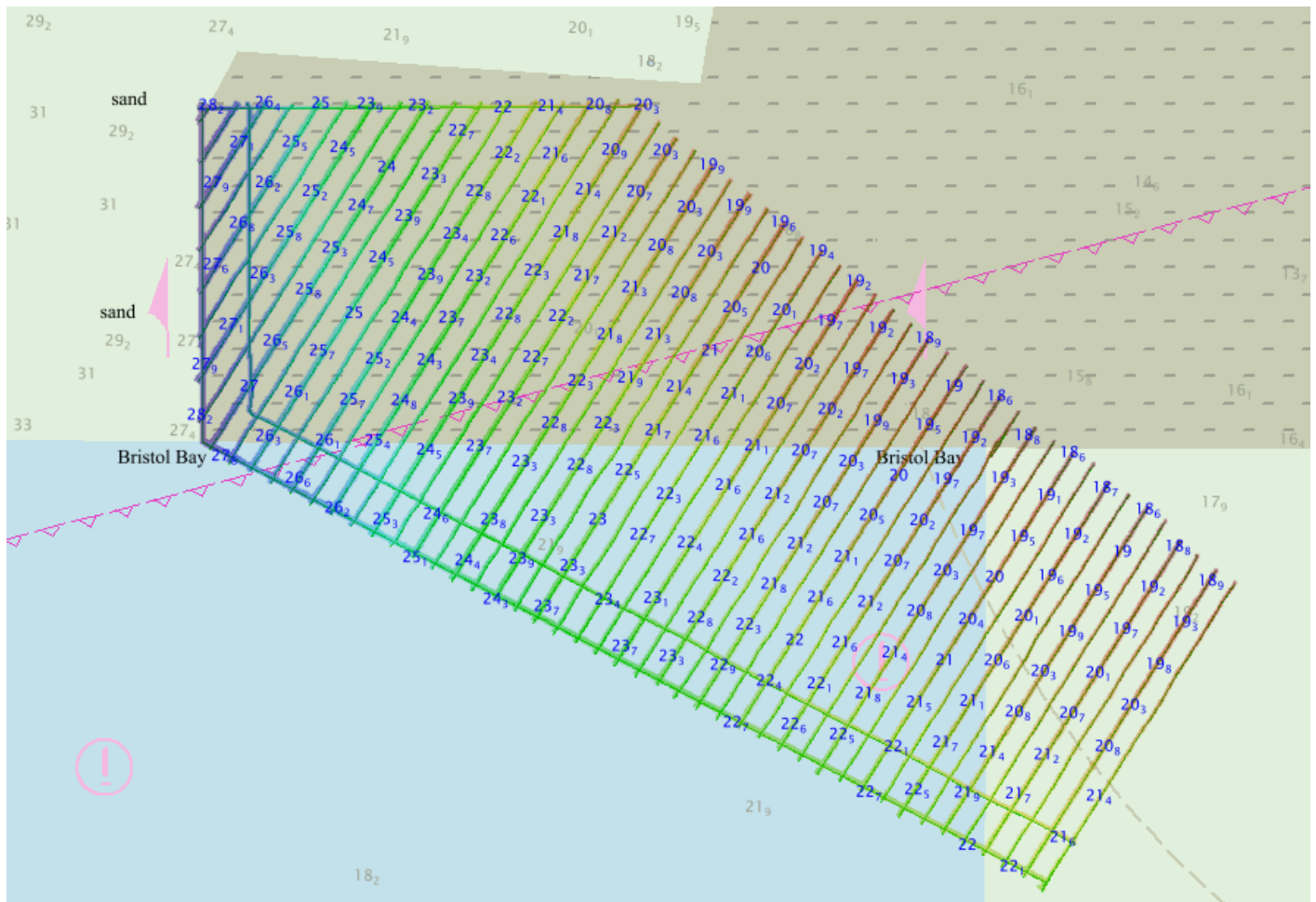
Figure 7: This survey overlaid on the largest scale ENCs. Soundings from this survey are blue. All soundings in meters.
