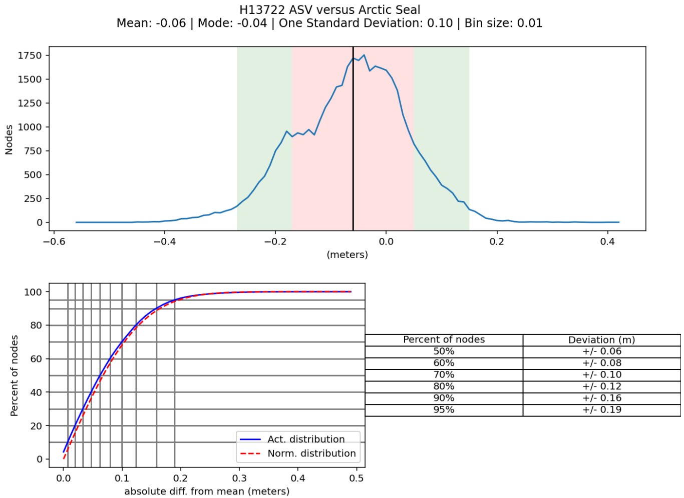
Figure 6: The results of the difference between ASV and Arctic Seal depth data for this survey.
