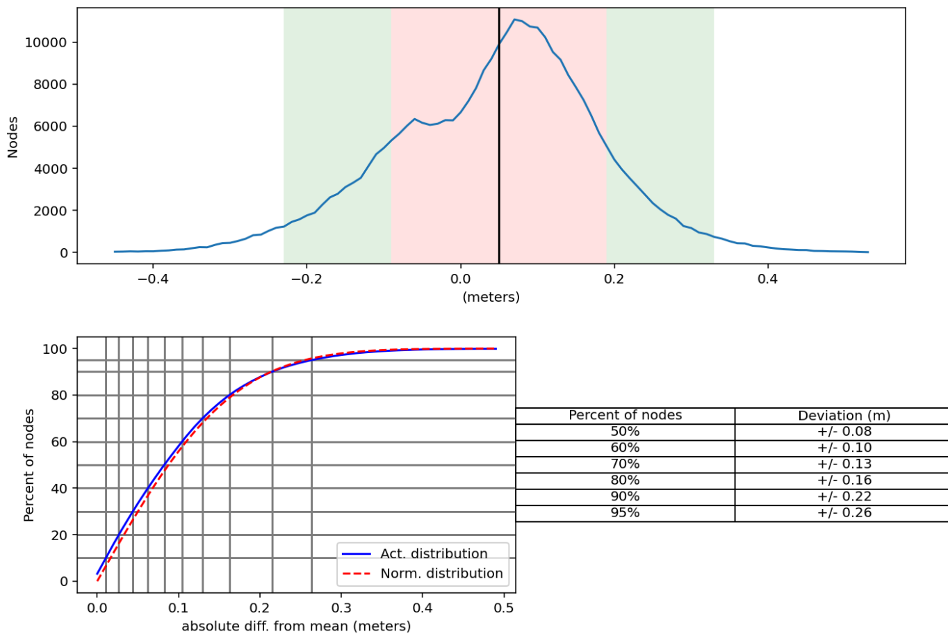
H13725 ASV versus Arctic Seal Depth Comparison Mean: 0.05 | Mode: 0.07 | One Standard Deviation: 0.13 | Bin size: 0.01
