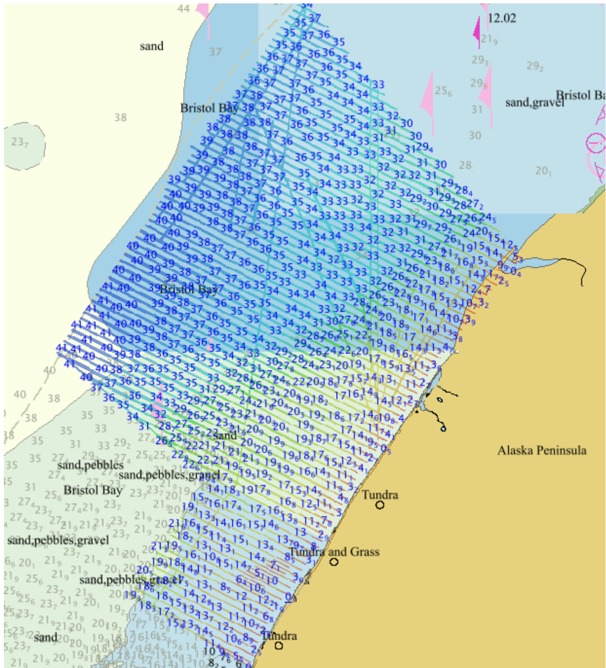
Figure 8: This survey overlaid on affected ENC. Soundings from this survey are blue. All soundings in meters.
