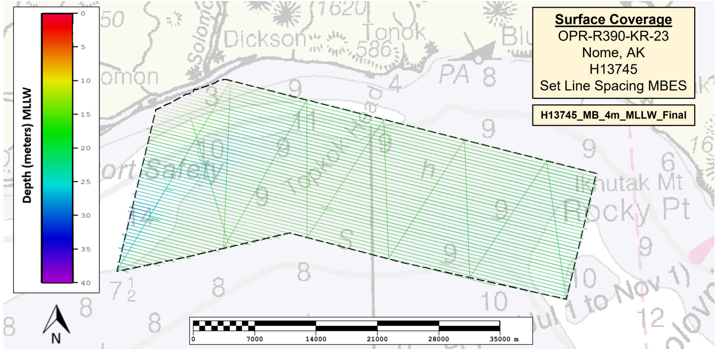
Figure 13: H13745 Finalized 4m CUBE weighted Dynamic Surface Coverage
