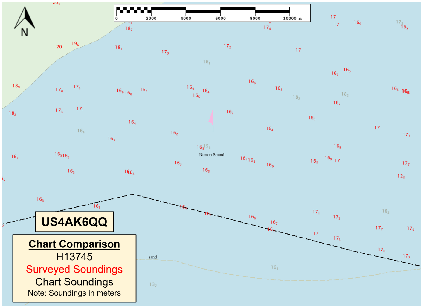
Figure 15: Generated Soundings used for Chart Comparison (US4AK6QQ)
