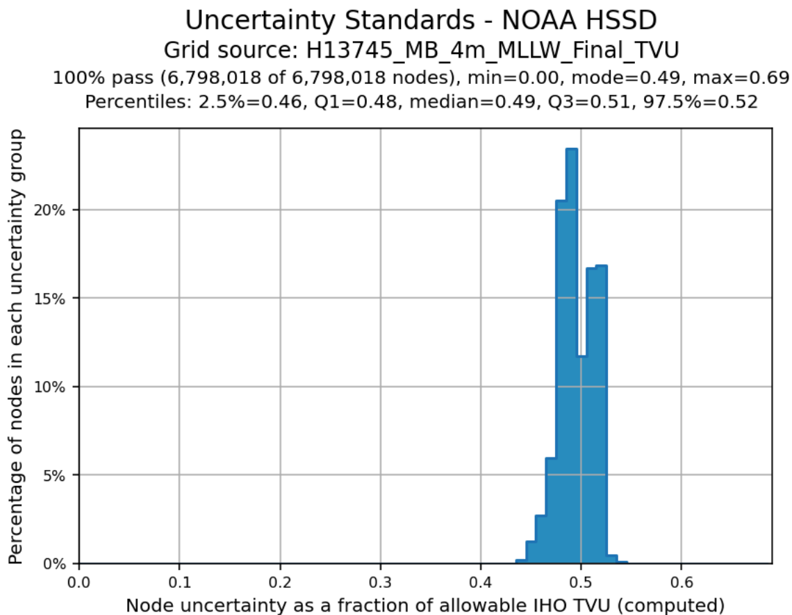
Figure 6: H13745 Finalized 4m MBES TVU Statistics
