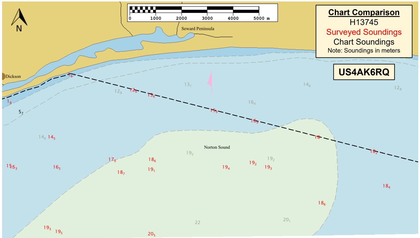
Figure 16: Generated Soundings used for Chart Comparison (US4AK6RQ)
