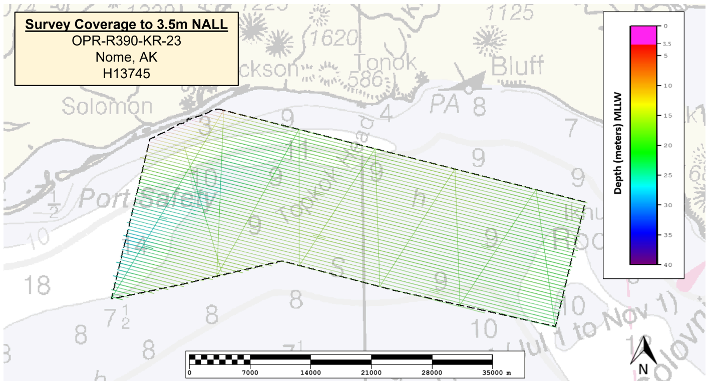
Figure 4: Survey Coverage with 3.5m NALL Displayed
