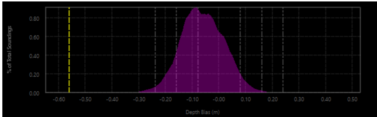
Figure 5: H13745 Crossline Comparison
