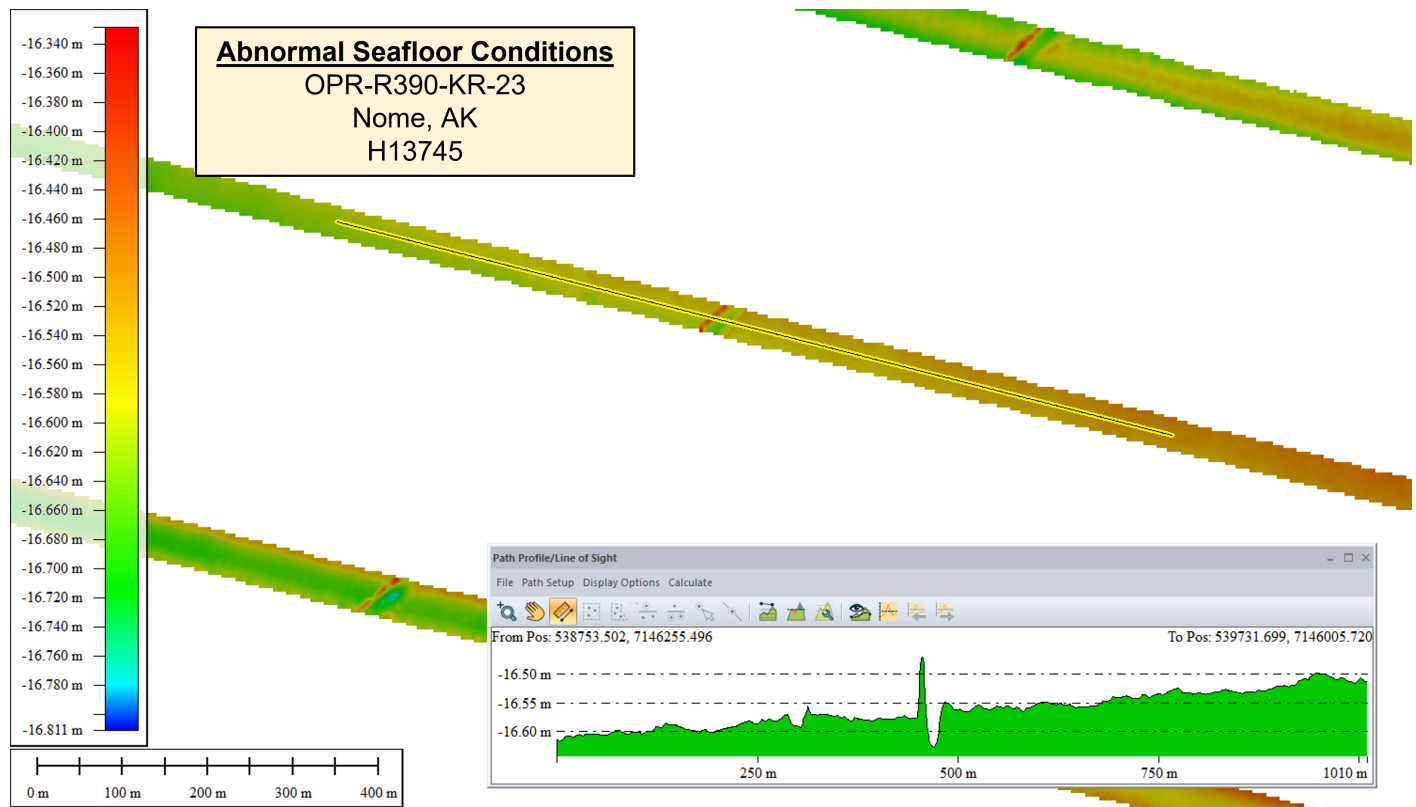
Figure 20: Abnormal Seafloor Condition (Ice Scour)
