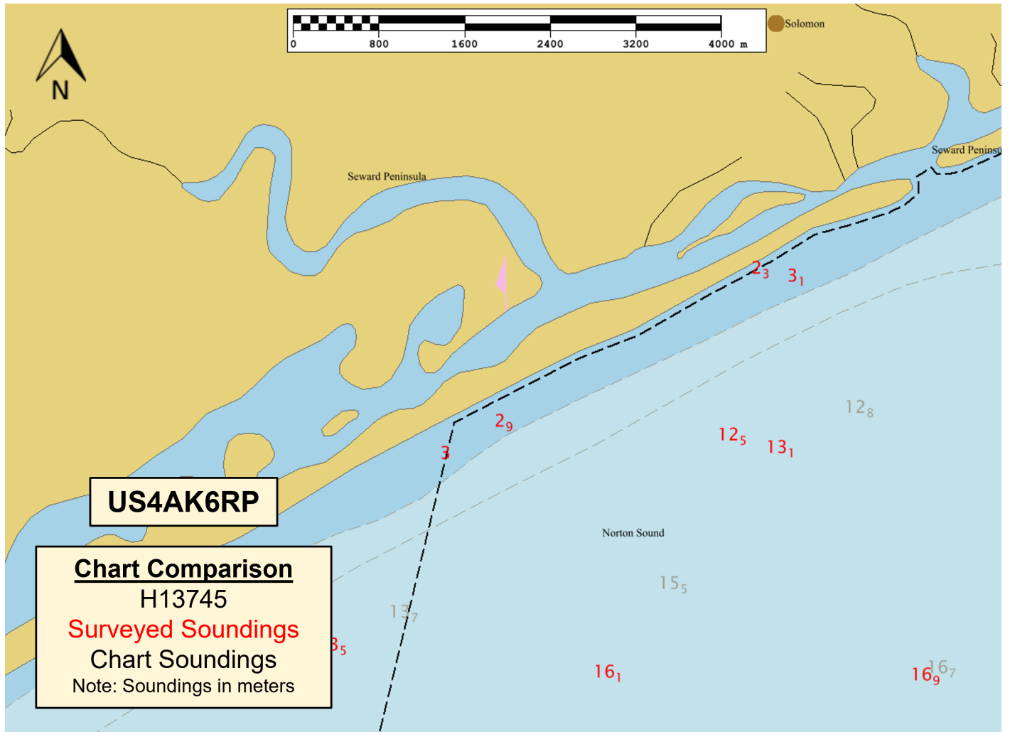
Figure 17: Generated Soundings used for Chart Comparison (US4AK6RP)
