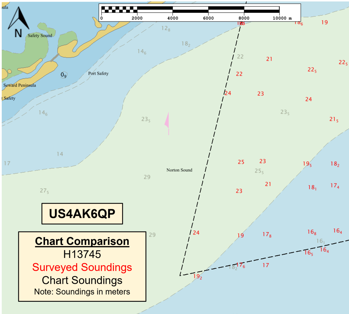
Figure 19: Generated Soundings used for Chart Comparison (US4AK6QP)
