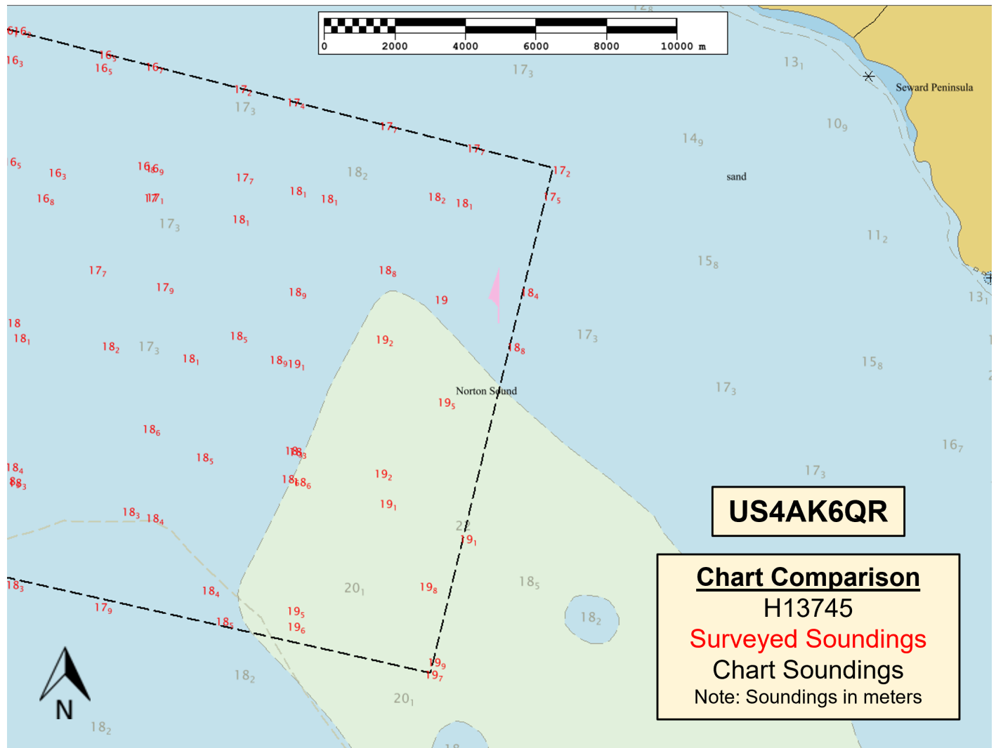
Figure 18: Generated Soundings used for Chart Comparison (US4AK6QR)
