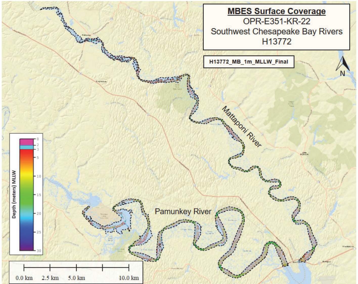
Figure 10: H13772 Finalized 1m CUBE Weighted Dynamic Surface Coverage
