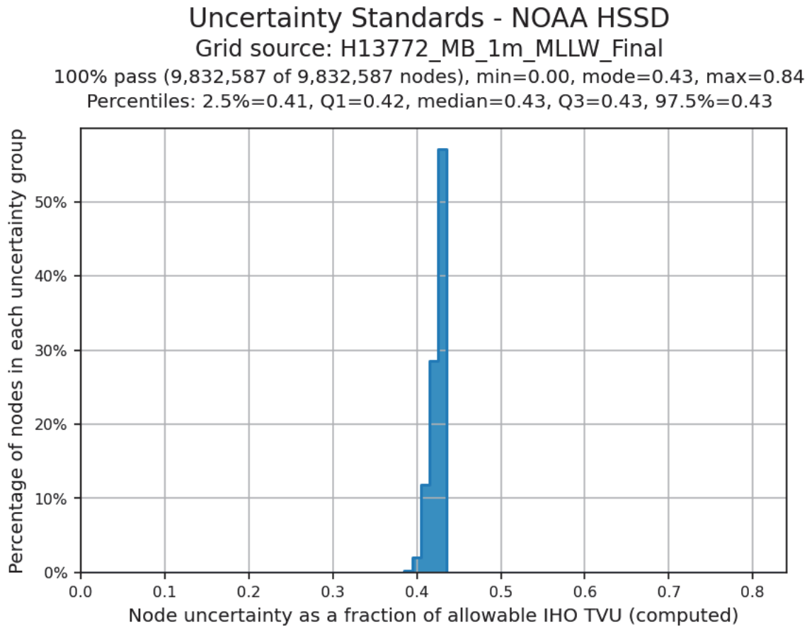
Figure 6: H13772 Finalized 1m MBES TVU Statistics
