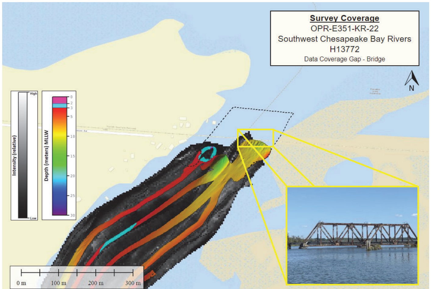
Figure 4: Coverage gap due to low bridge clearance
