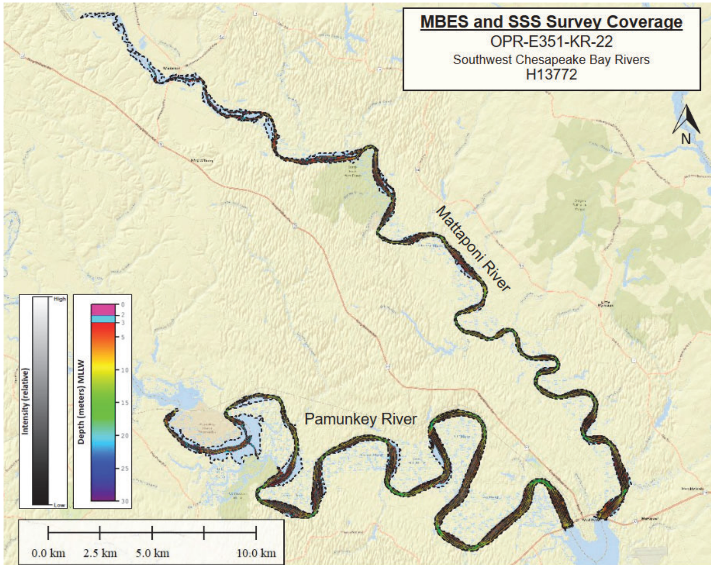
Figure 3: Survey Coverage with combined MBES and SSS
