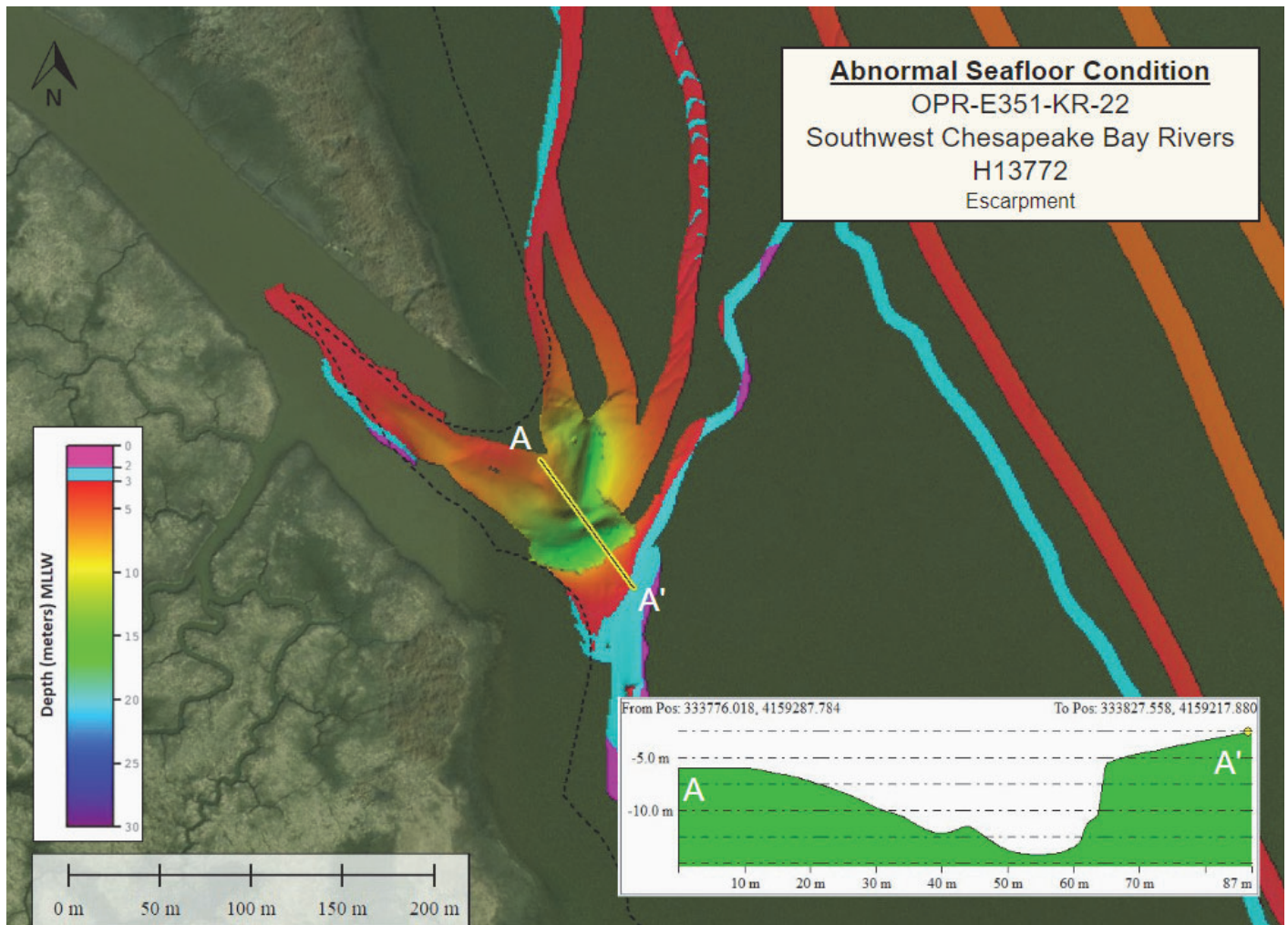
Figure 14: Abnormal Seafloor Condition observed in Pamunkey River
