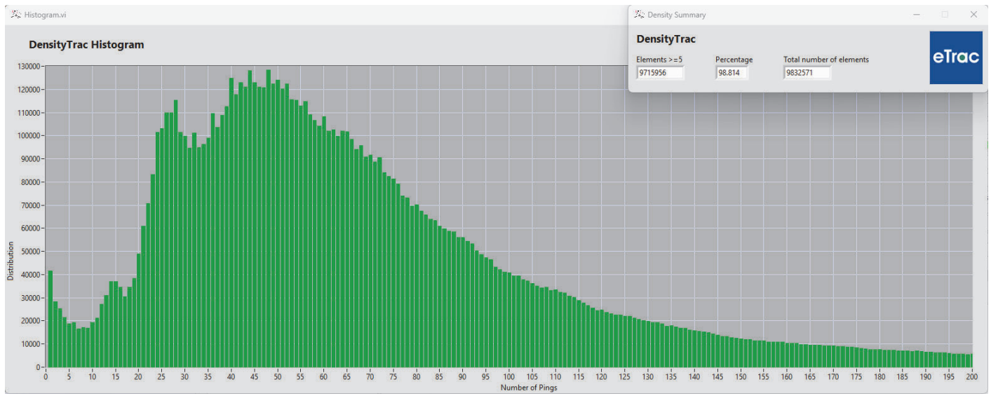
Figure 9: H13772 Finalized 1m Set Line Spacing MBES Density Distribution
