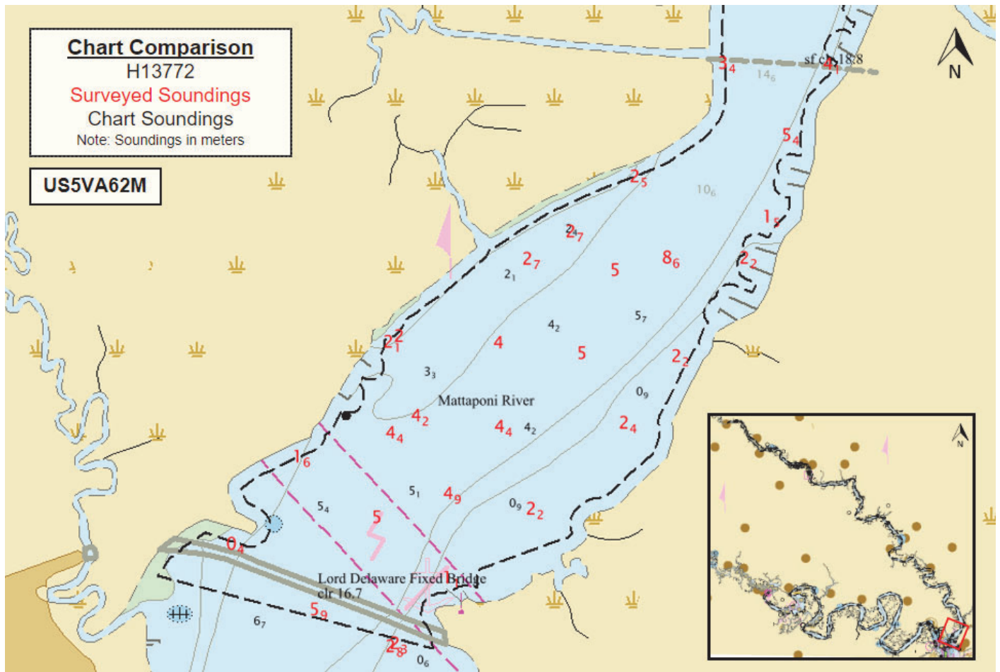
Figure 13: Generated Soundings used for Chart Comparison (US5VA62M)
