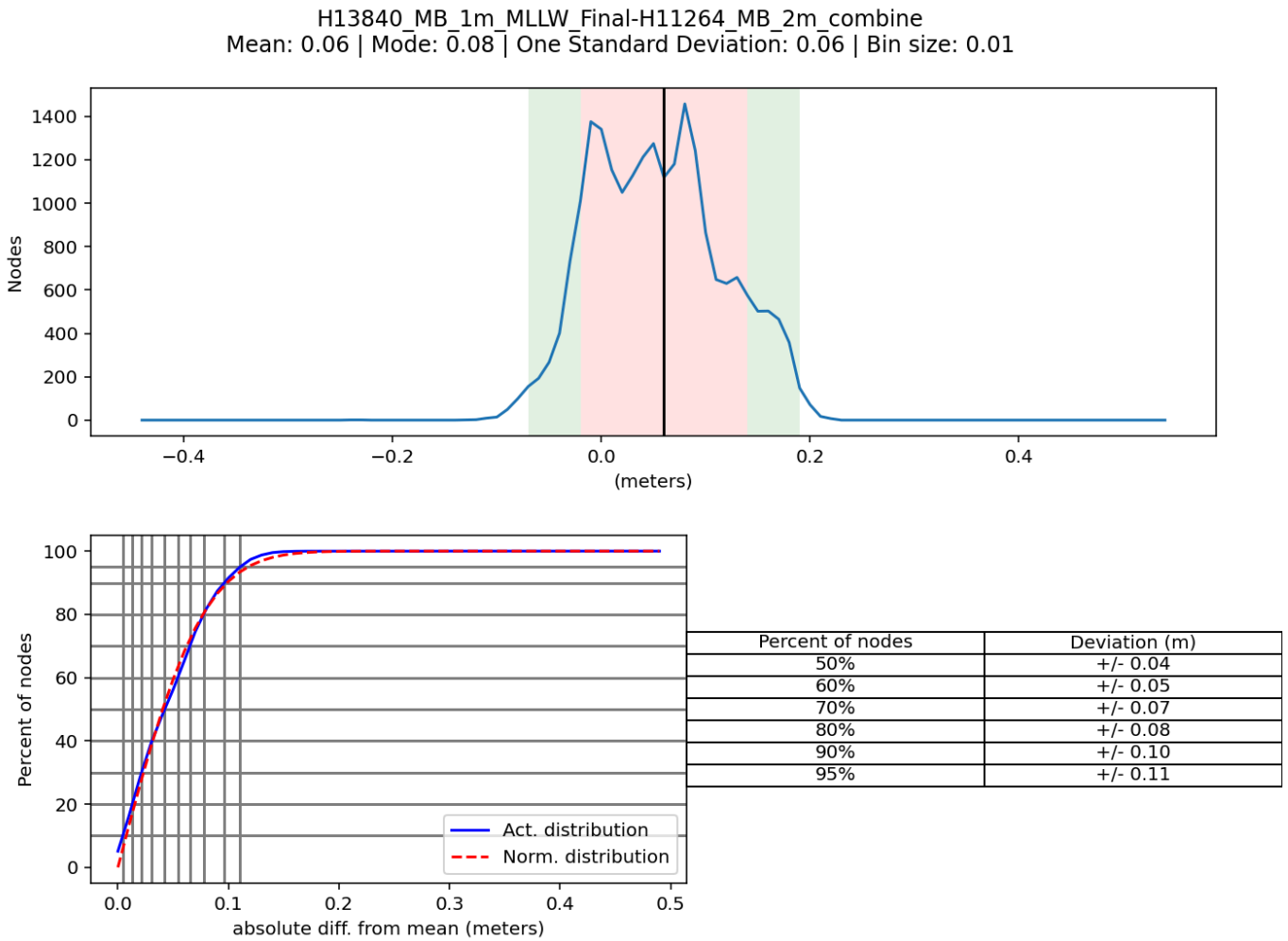
Figure 8: Distribution summary plot of survey H13840 1-meter vs H11624 2-meter
