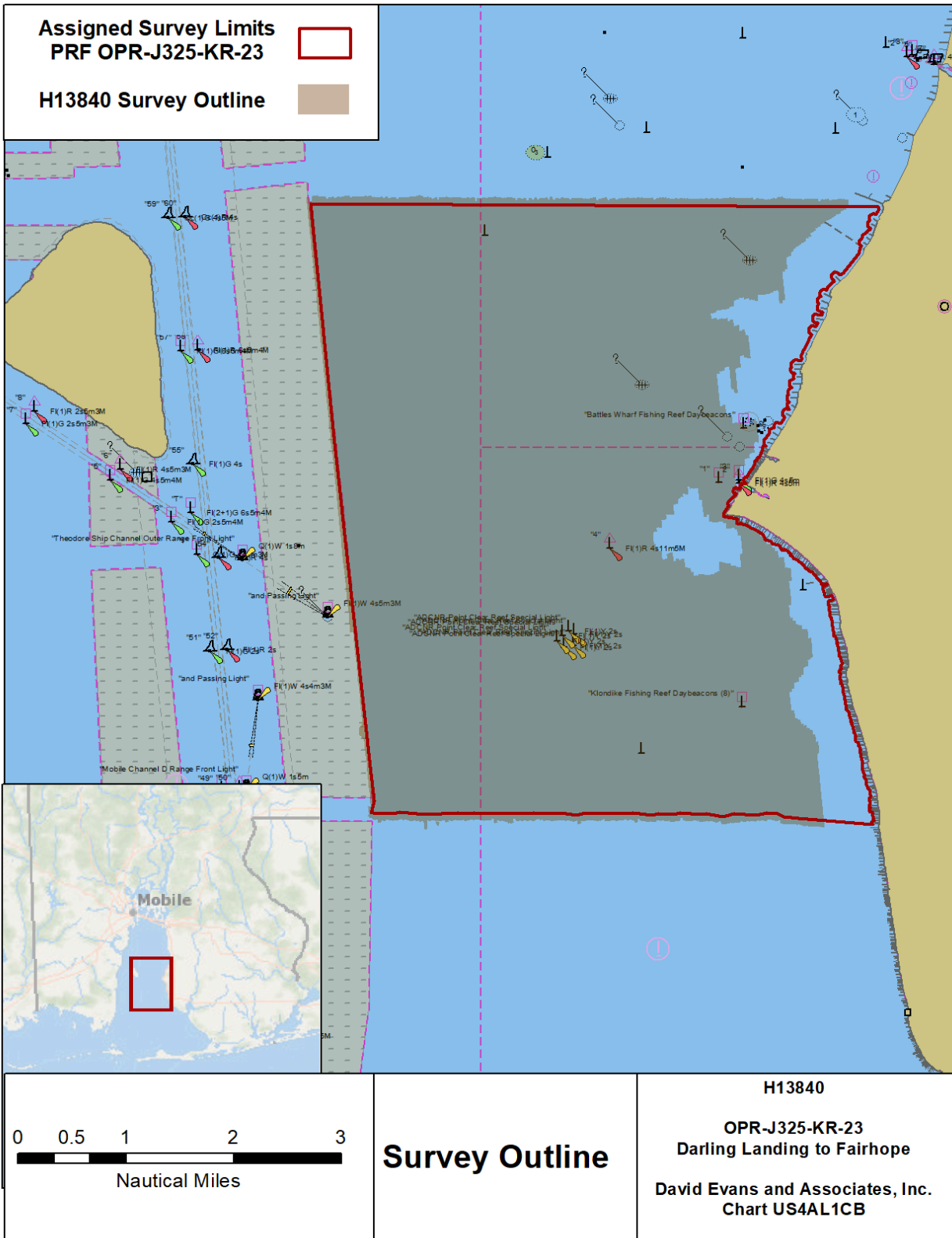
Figure 2: H13840 Survey Outline
