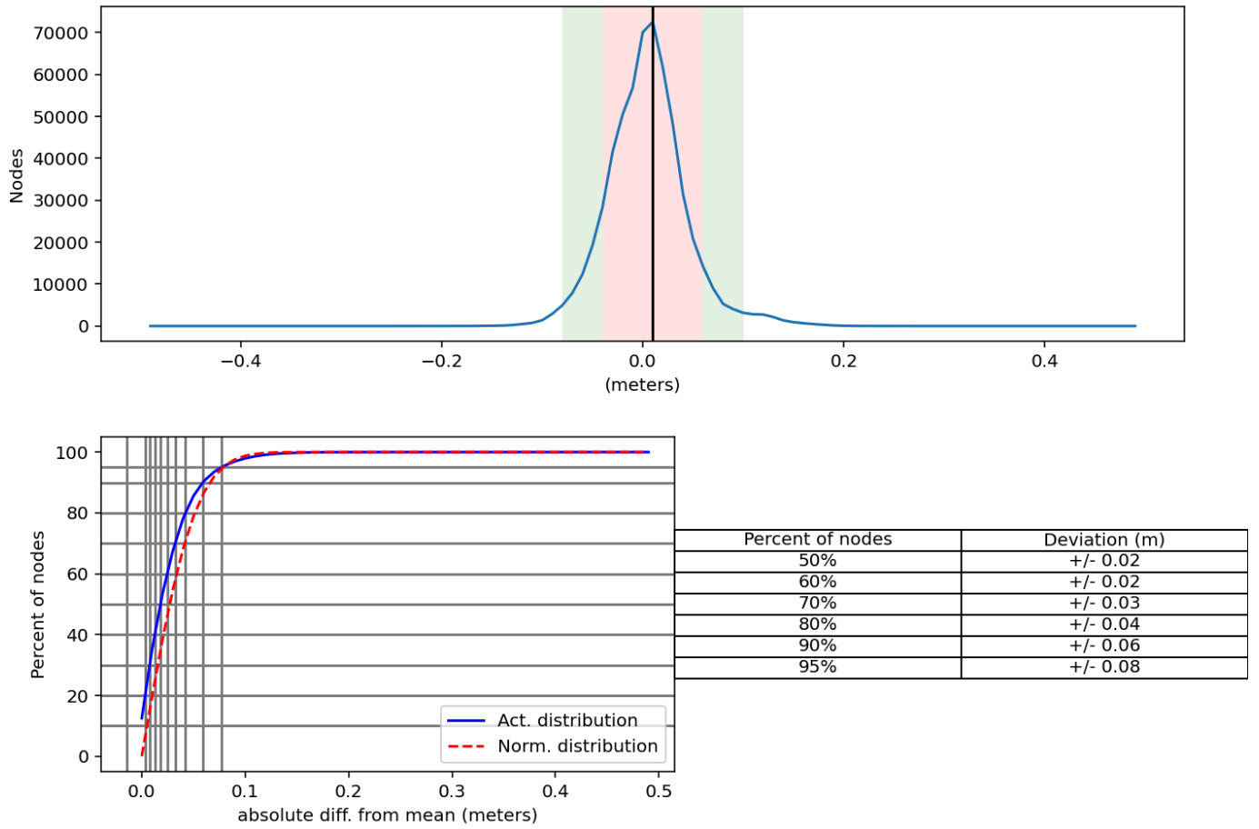
Figure 7: Distribution summary plot of survey H13840 1-meter vs H13837 1-meter
