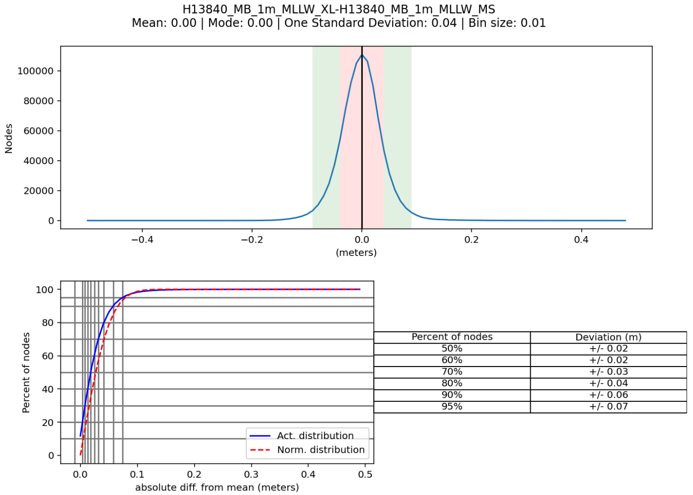
Figure 4: H13840 Crossline Difference
