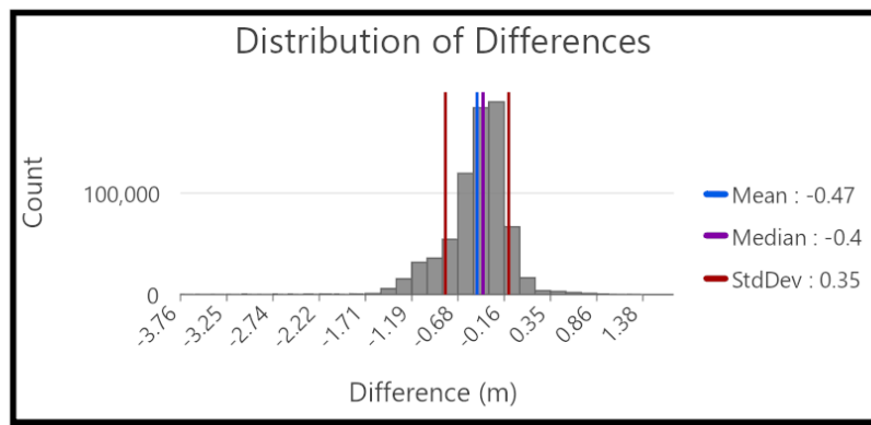
Figure 11: Depth Difference Between H13840 and Band 5 ENC
