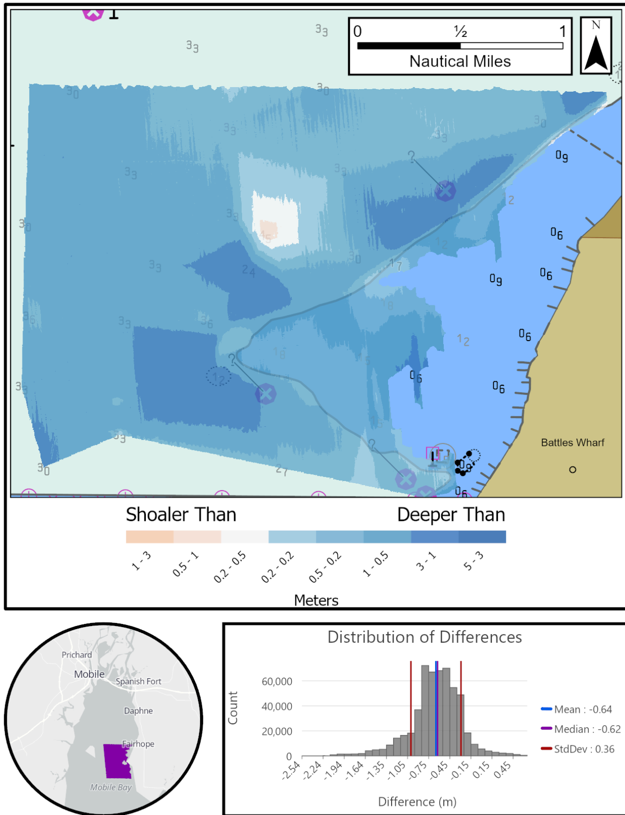
Figure 10: Depth Difference Between H13840 and Band 4 ENC
