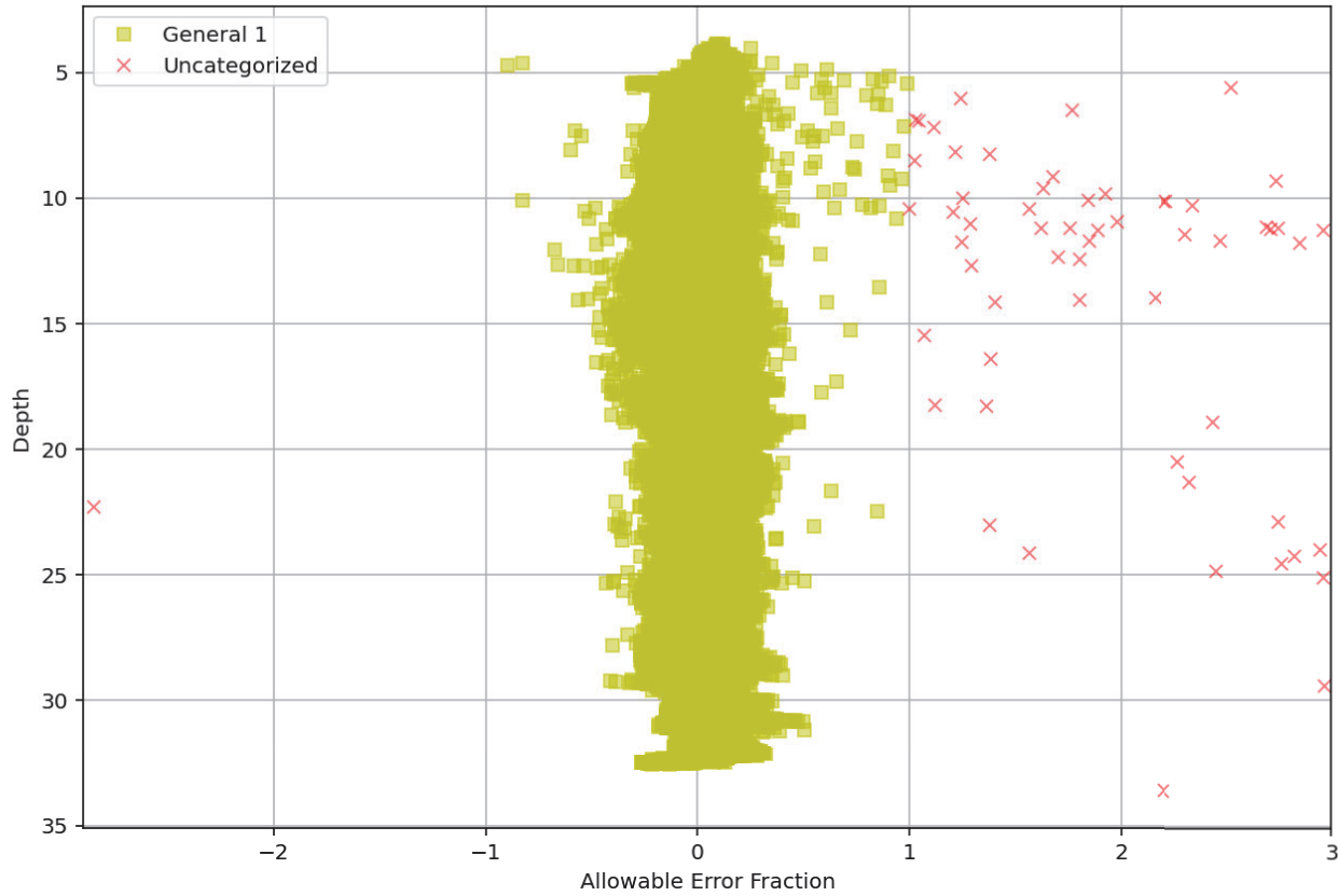
Pydro derived plot showing percentage-pass value of H13868 mainscheme to crossline data.
