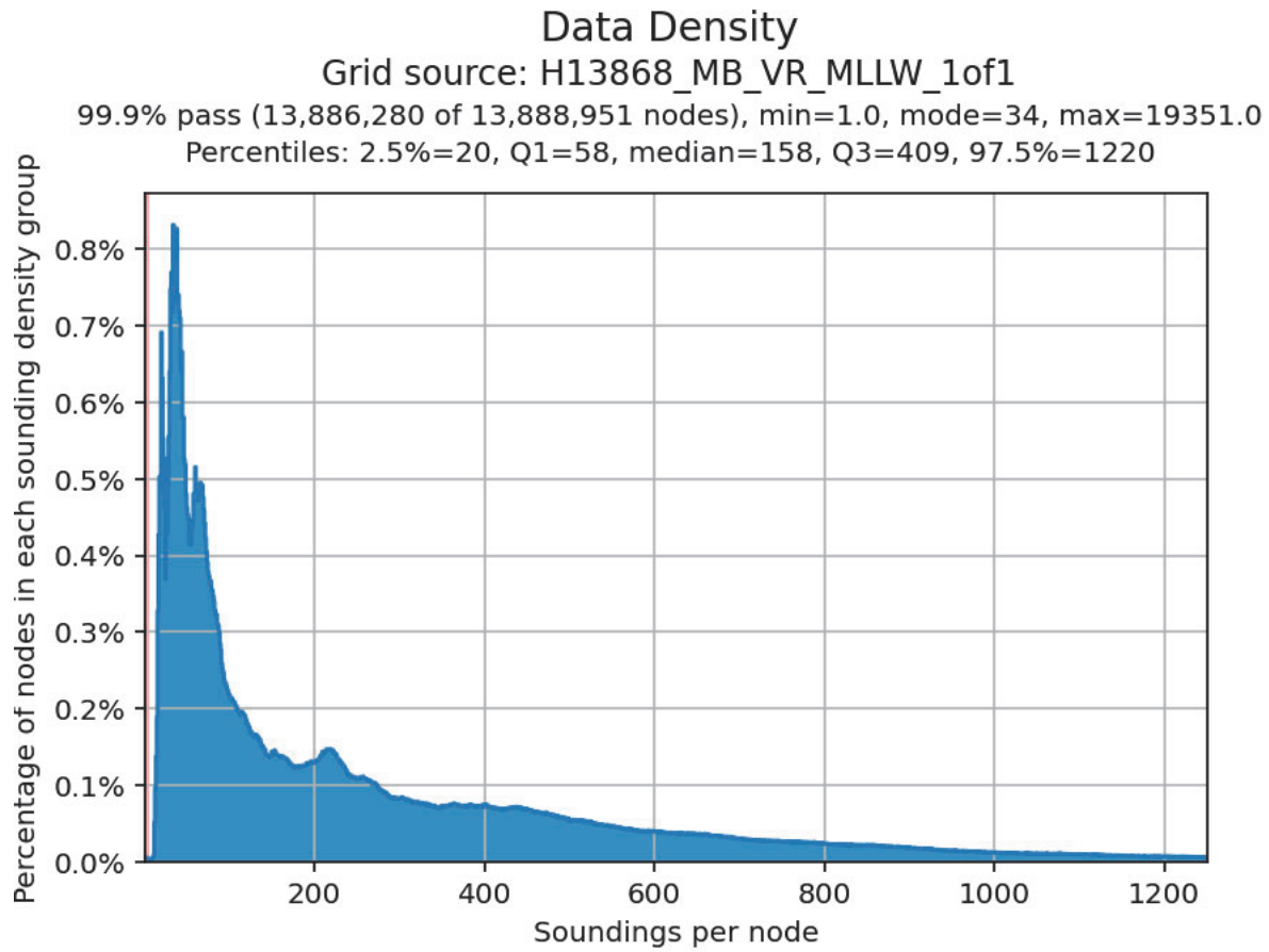
Pydro Grid QA derived histogram plot showing HSSD density requirements of H13868 finalized variable-resolution MBES data.
