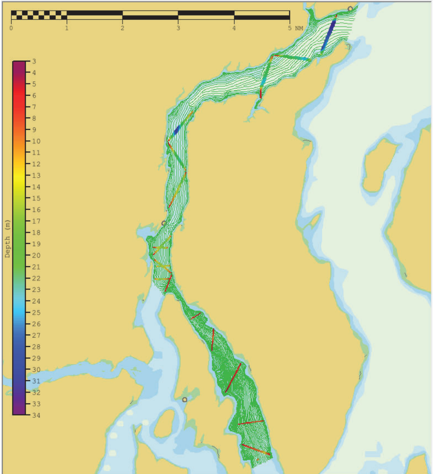
H13868 crossline surface colored by depth overlaid on mainscheme tracklines.
