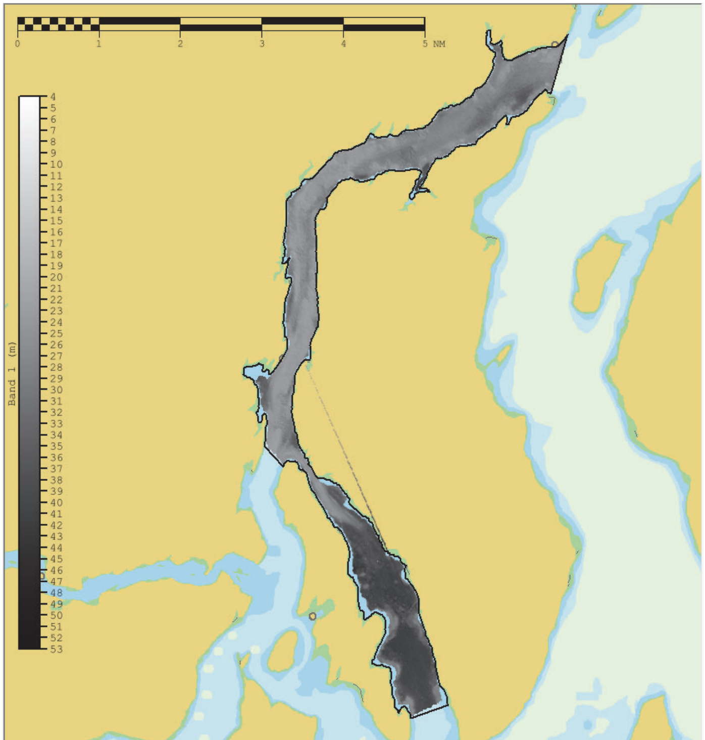
H13868 backscatter mosaic created in FMGT (v.7.11.1)
