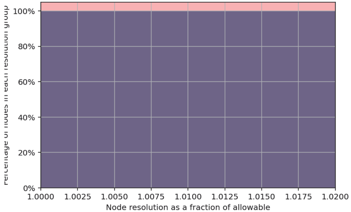
Pydro Grid QA derived histogram plot showing HSSD resolution requirements of H13868 finalized variable-resolution MBES data.
