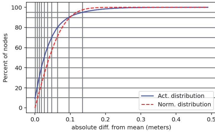
Pydro derived plot showing absolute difference statistics of the junction between H13866 and H13868 variable resolution surface.
