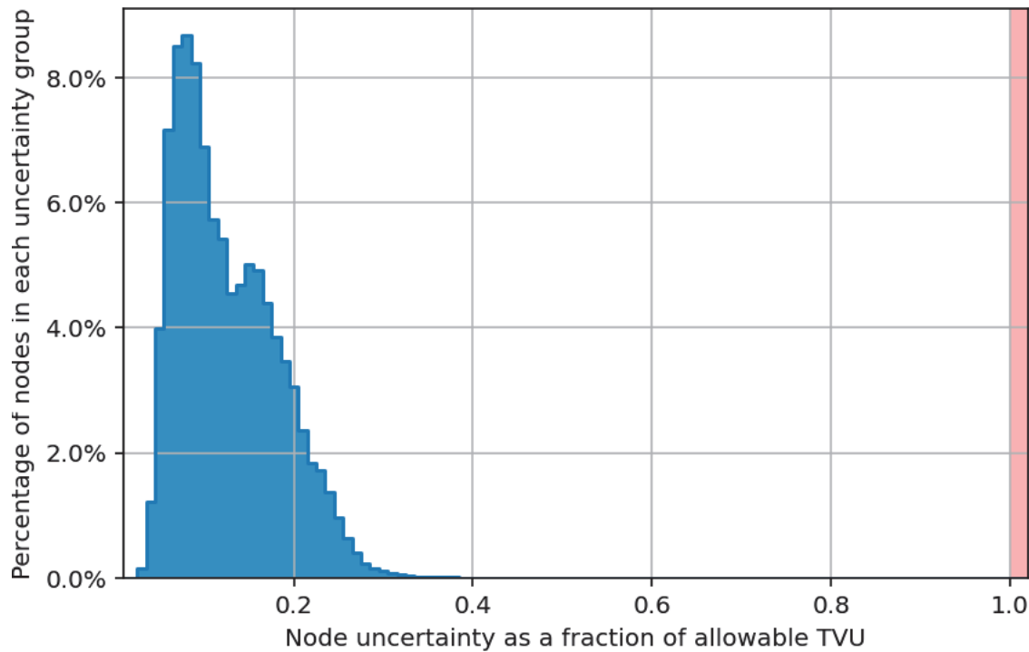
Pydro Grid QA derived histogram plot showing HSSD uncertainty requirements of H13868 finalized variable-resolution MBES data.
