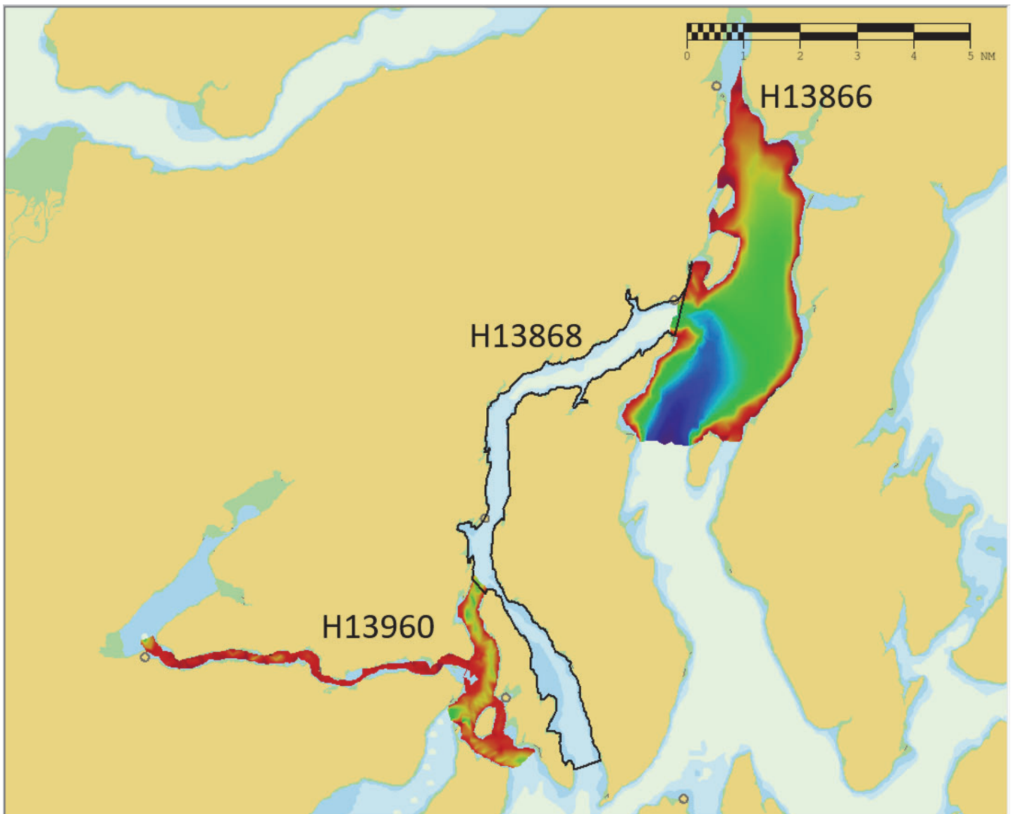
Junction surface H13868 with H13866 survey extents.
