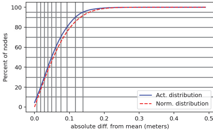
Pydro derived plot showing absolute difference statistics of H13868 mainscheme to crossline data.
