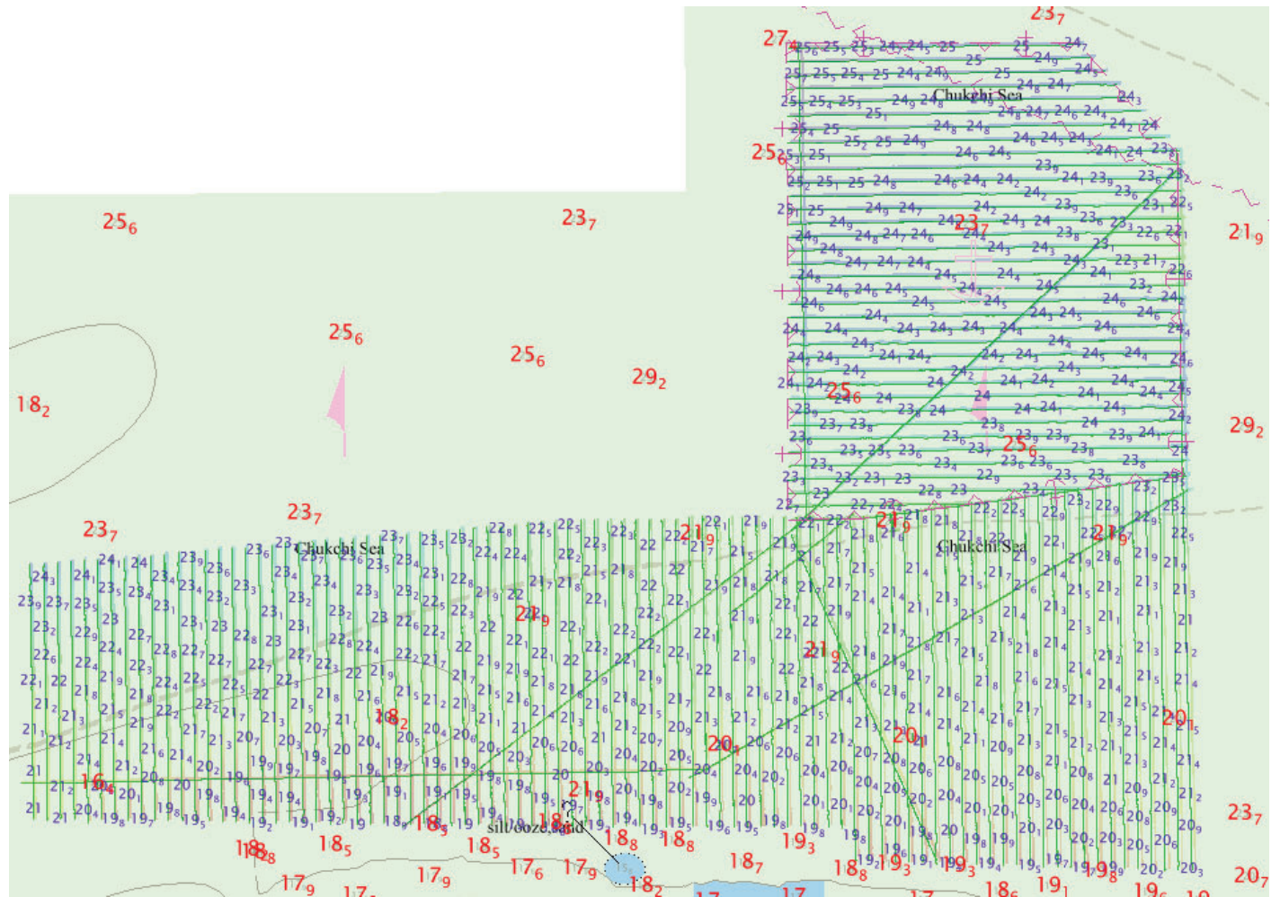
Figure 7: This survey overlaid on affected large scale ENCs. Soundings from this survey are blue. All soundings in meters.
