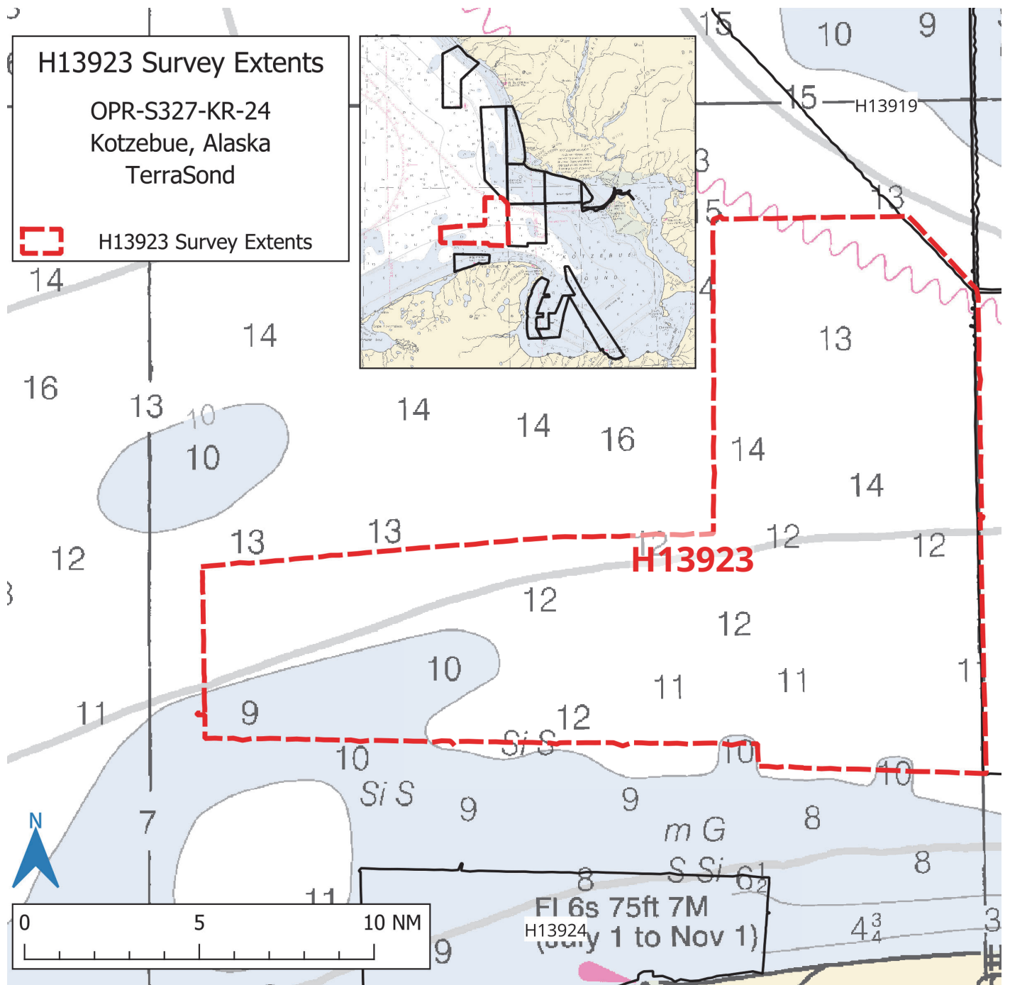
Figure 1: Figure showing the survey extents.
