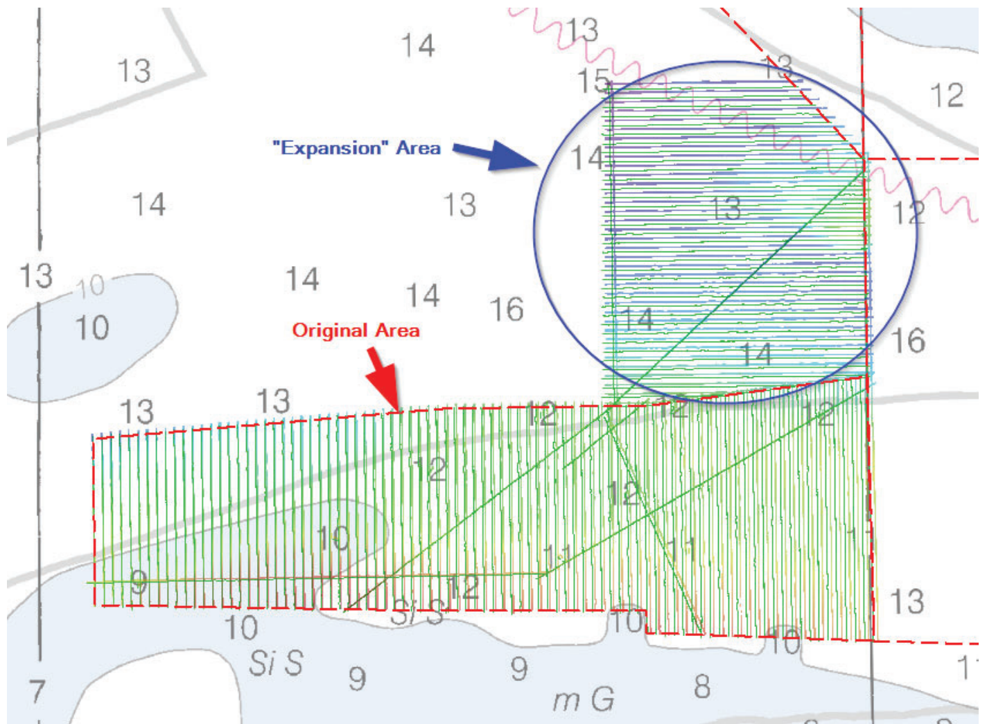
Figure 2: Figure showing the originally assigned survey area and the approximate extents of the 65 SQNM "expansion" of this sheet.
