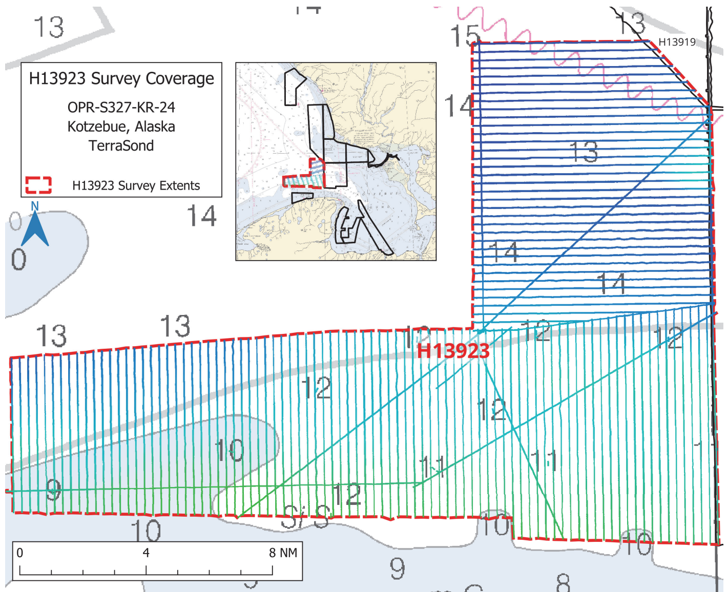
Figure 3: Figure showing coverage achieved on this survey.
