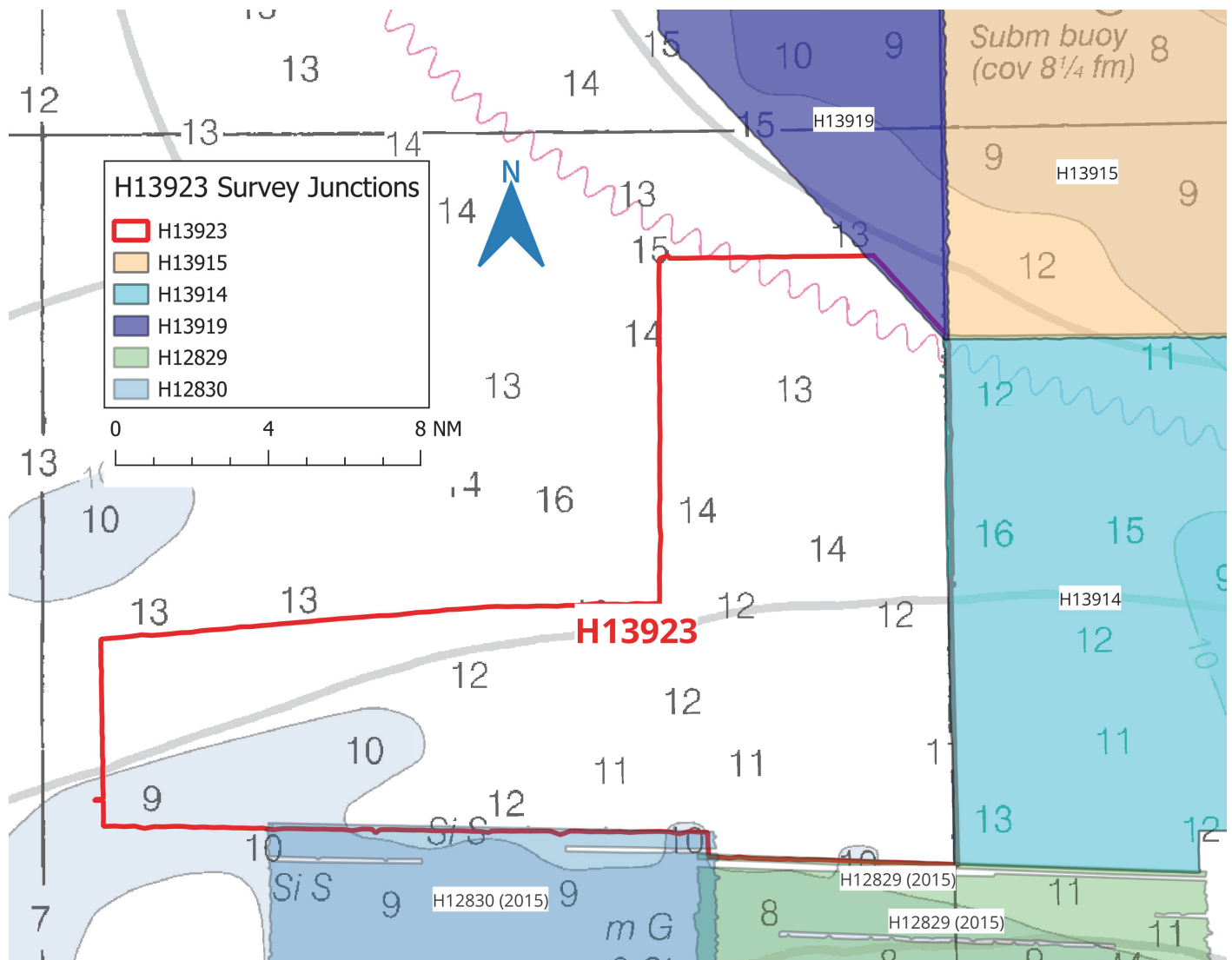
Figure 6: Figure showing survey junctions.
