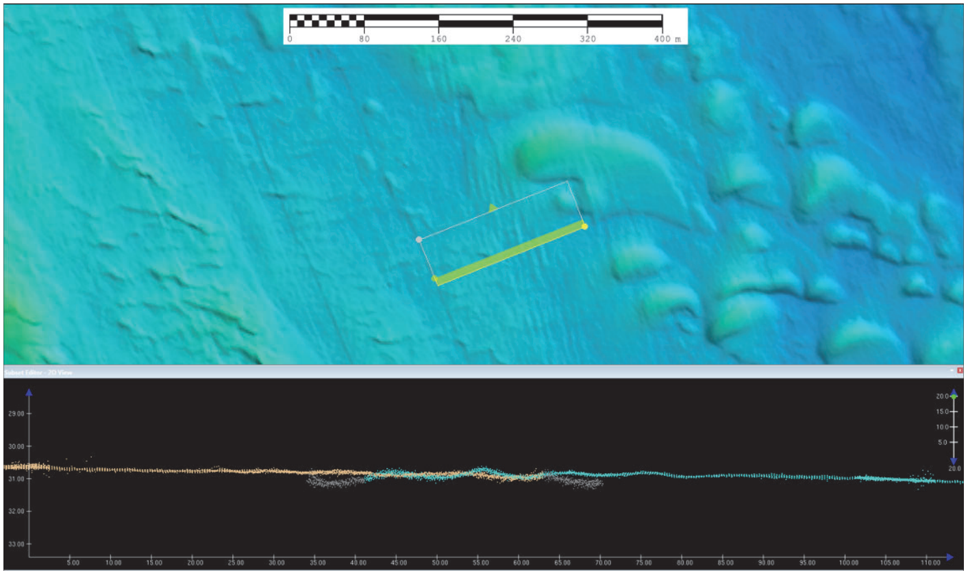
Figure 20: H13943 surface artifacts as a result of refraction causing outer beam noise
