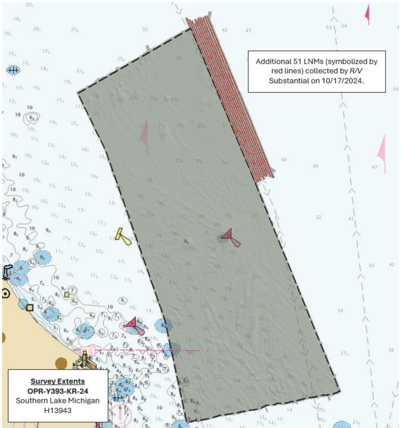
Figure 3: H13943 extents of additional coverage past survey limits as part of CLIN2 for this project, overlaid onto Charts US4IL1YX, US4IL1YY, and US5CHILL
