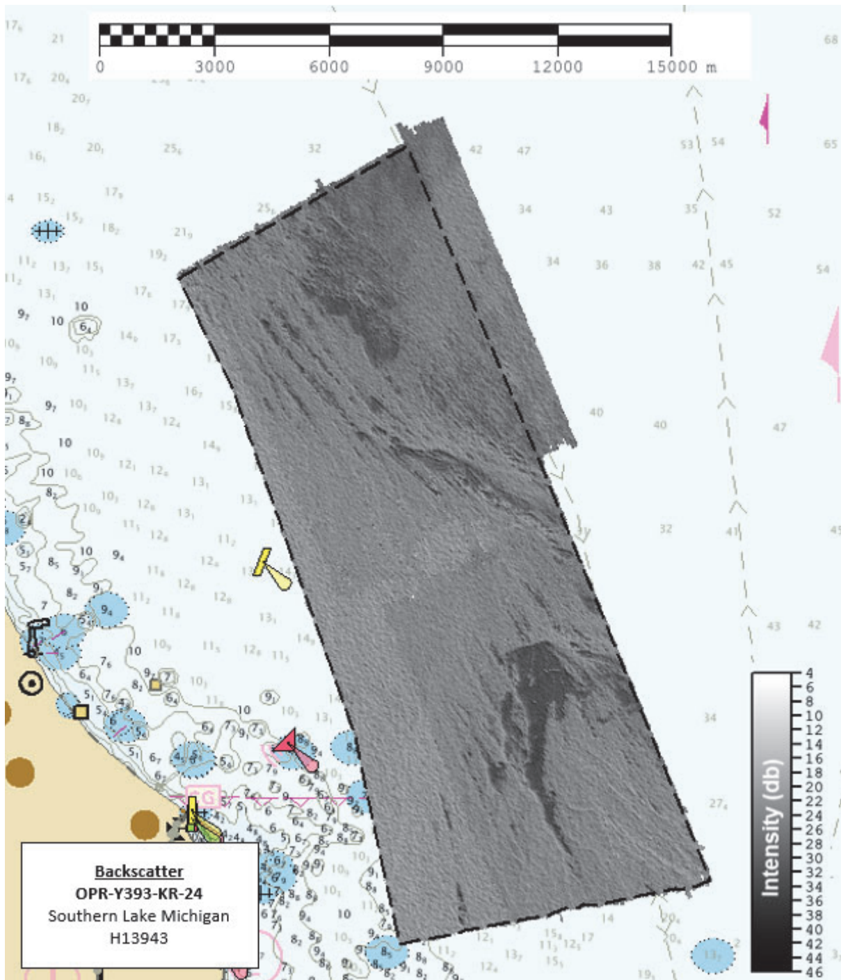
Figure 24: H13943 combined backscatter coverage
