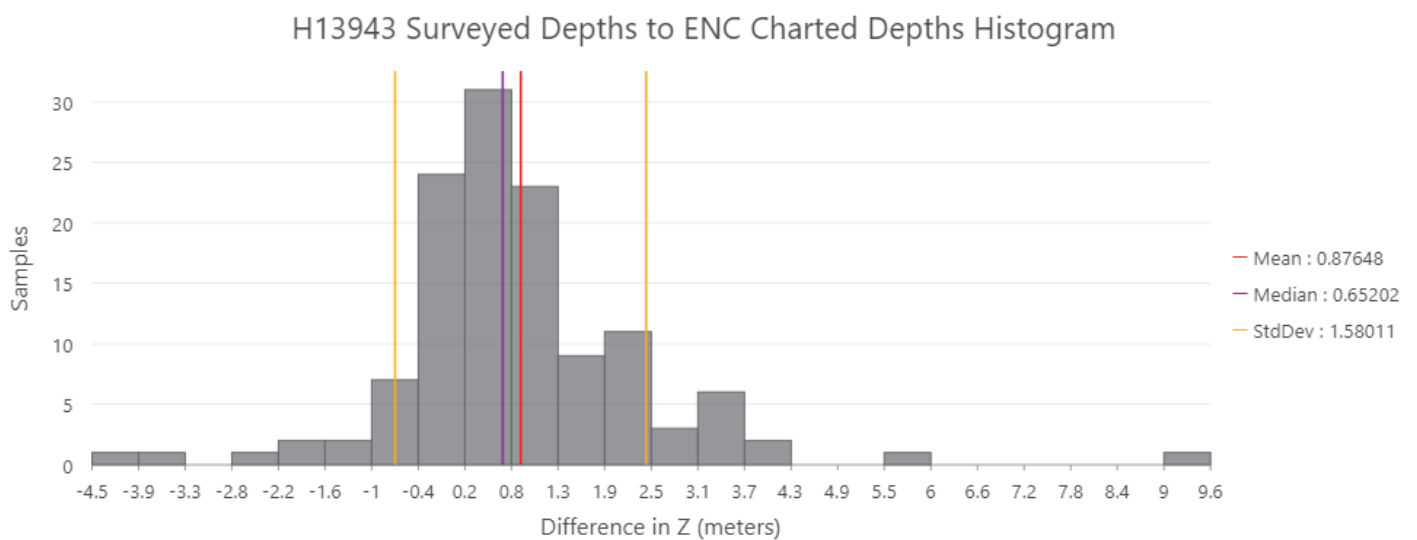
Figure 26: H13943 statistical analysis of surveyed depths to charted soundings
