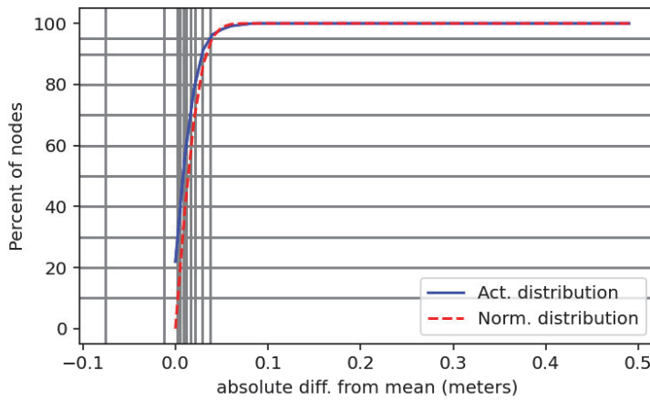
Figure 10: Junction analysis between H13943 and H13942 Finalized 1 m MBES CUBE surface
