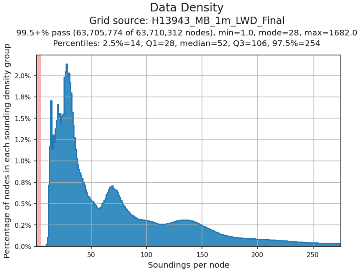
Figure 21: Finalized 1 m CUBE surface density statistics for H13943
