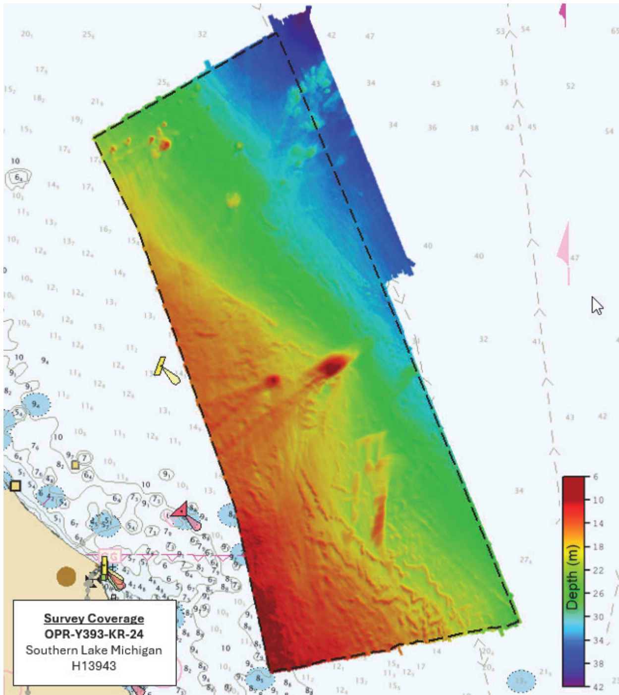
Figure 4: H13943 survey coverage overlaid onto Charts US4IL1YX, US4IL1YY, and US5CHILL
