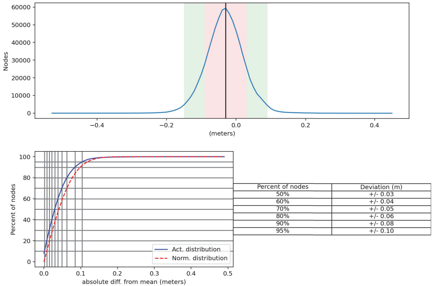
Figure 17: Junction analysis between H13943 and H13815 2 m MBES CUBE surface
