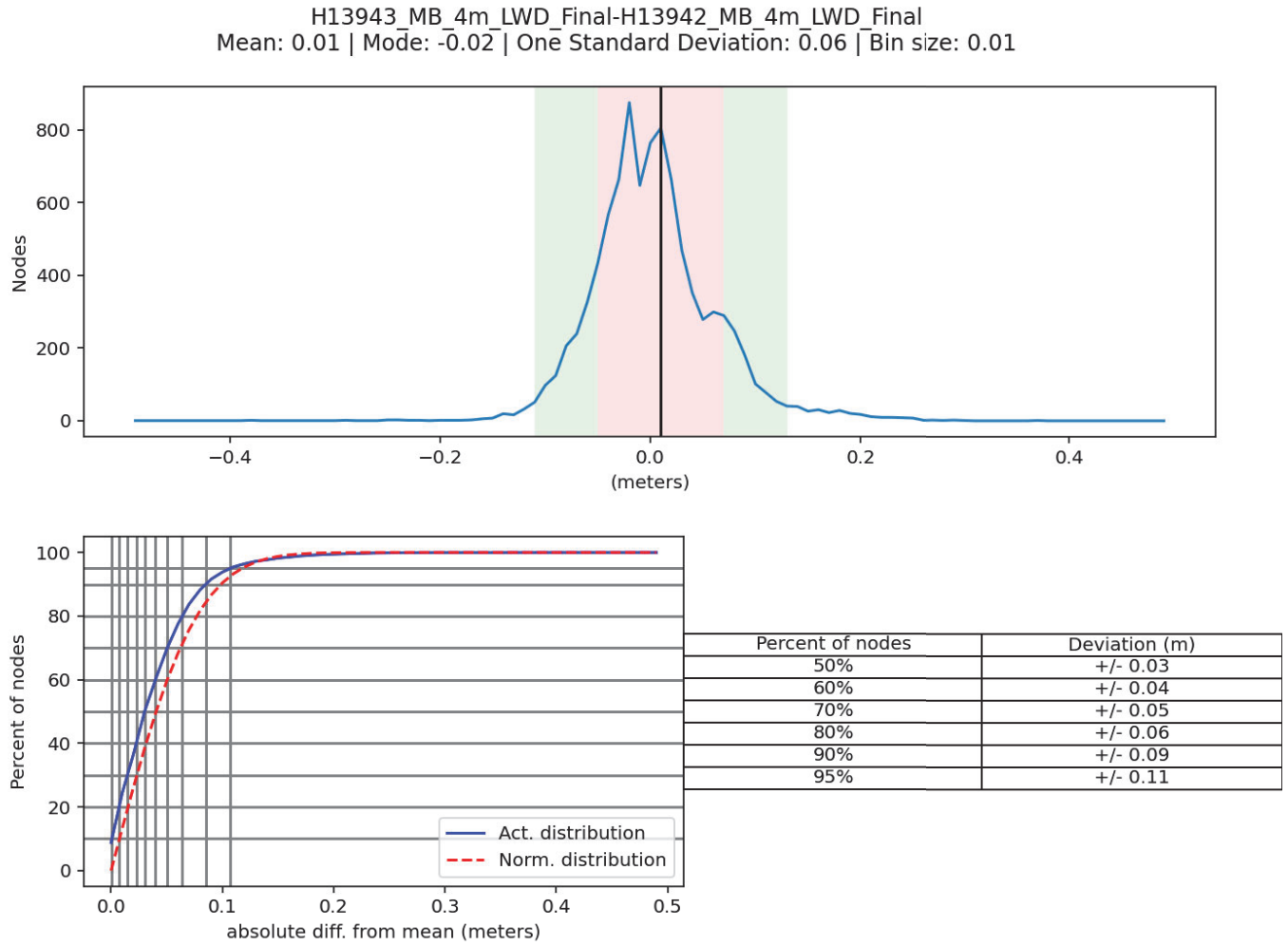
Figure 12: Junction analysis between H13943 and H13942 Finalized 4 m MBES CUBE surface
