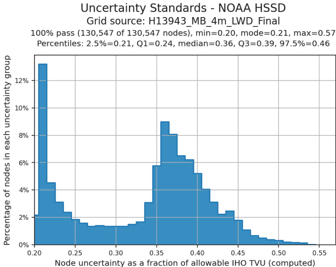
Figure 8: Finalized 4 m CUBE surface TVU statistics for H13943
