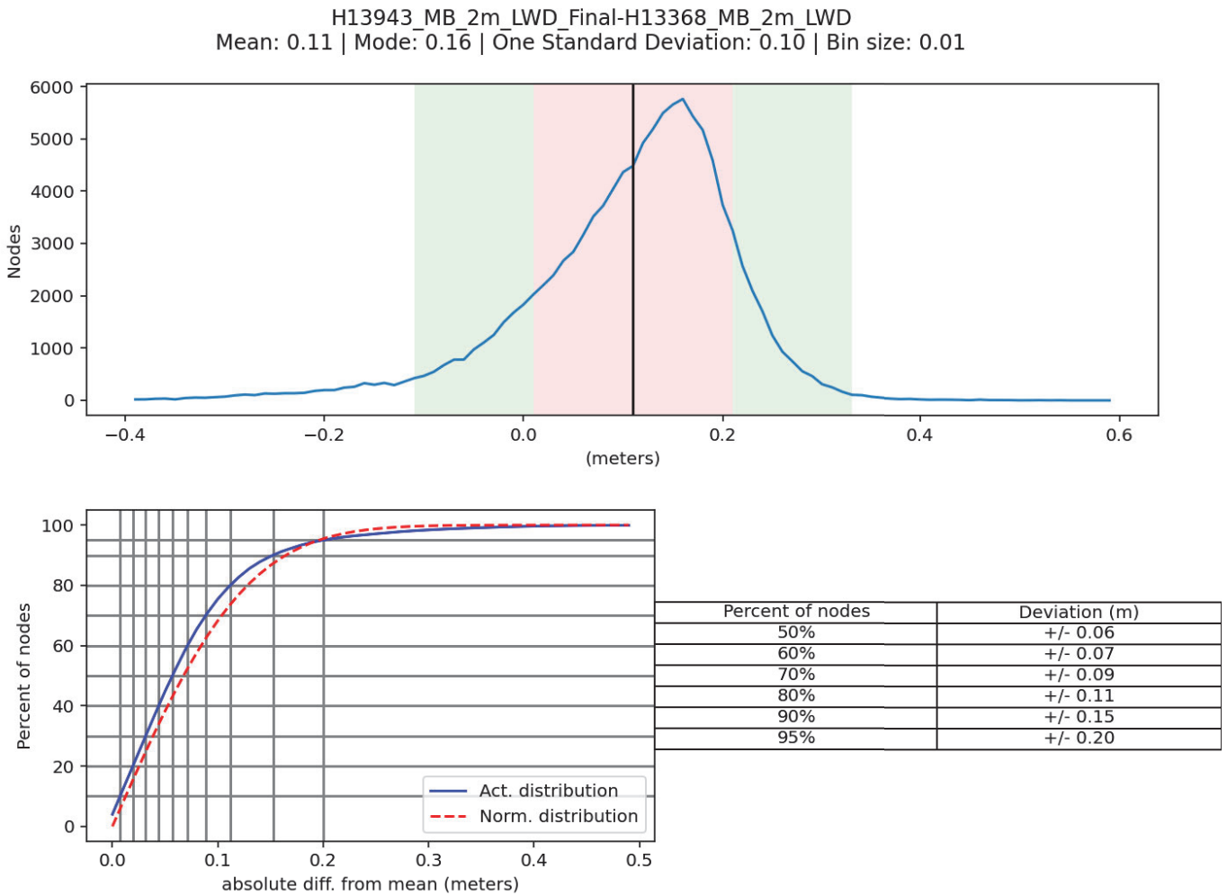
Figure 15: Junction analysis between H13943 and H13368 Finalized 2 m MBES CUBE surface
