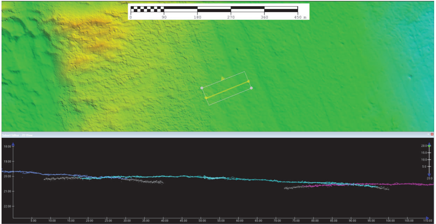
Figure 19: H13943 surface artifacts as a result of refraction causing the soundings to trend concave / convex
