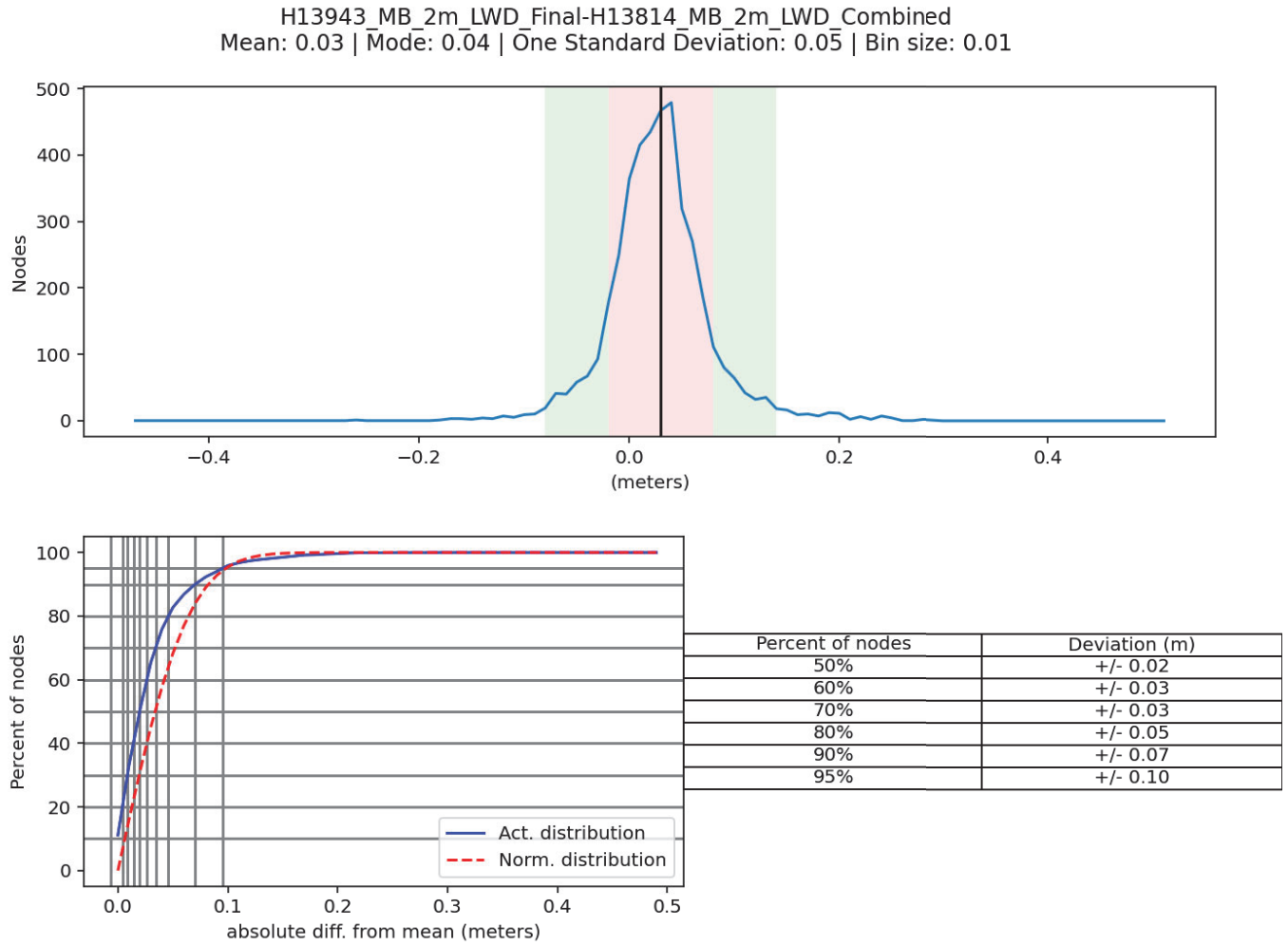
Figure 16: Junction analysis between H13943 and H13814 Finalized 2 m MBES CUBE surface
