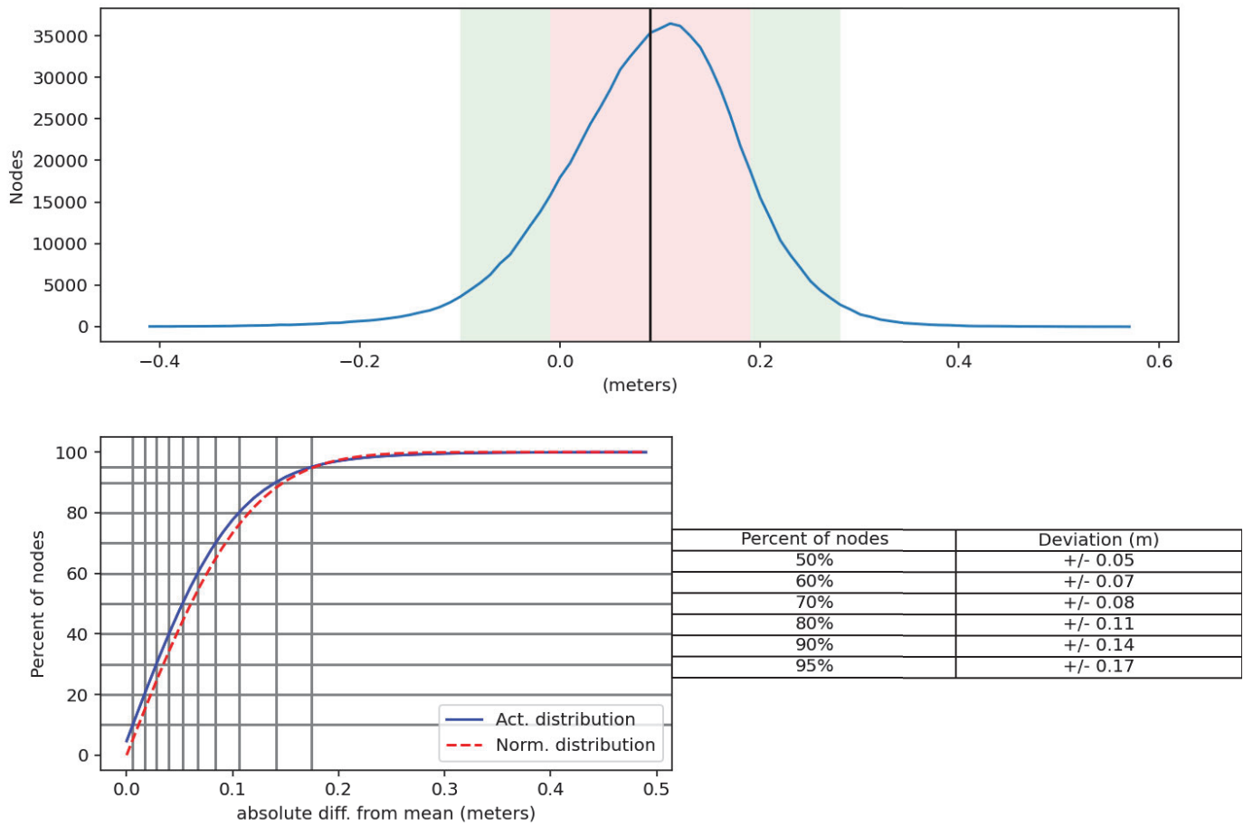
Figure 14: Junction analysis between H13943 and H13368 Finalized 1 m MBES CUBE surface
