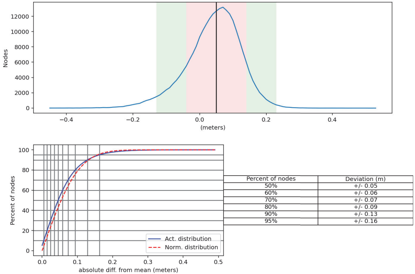
Figure 13: Junction analysis between H13943 and H13364 Finalized 1 m MBES CUBE surface
