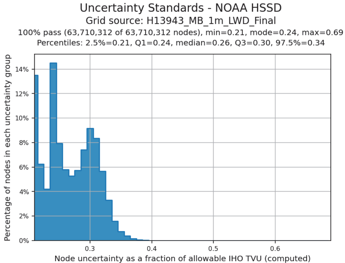
Figure 6: Finalized 1 m CUBE surface TVU statistics for H13943
