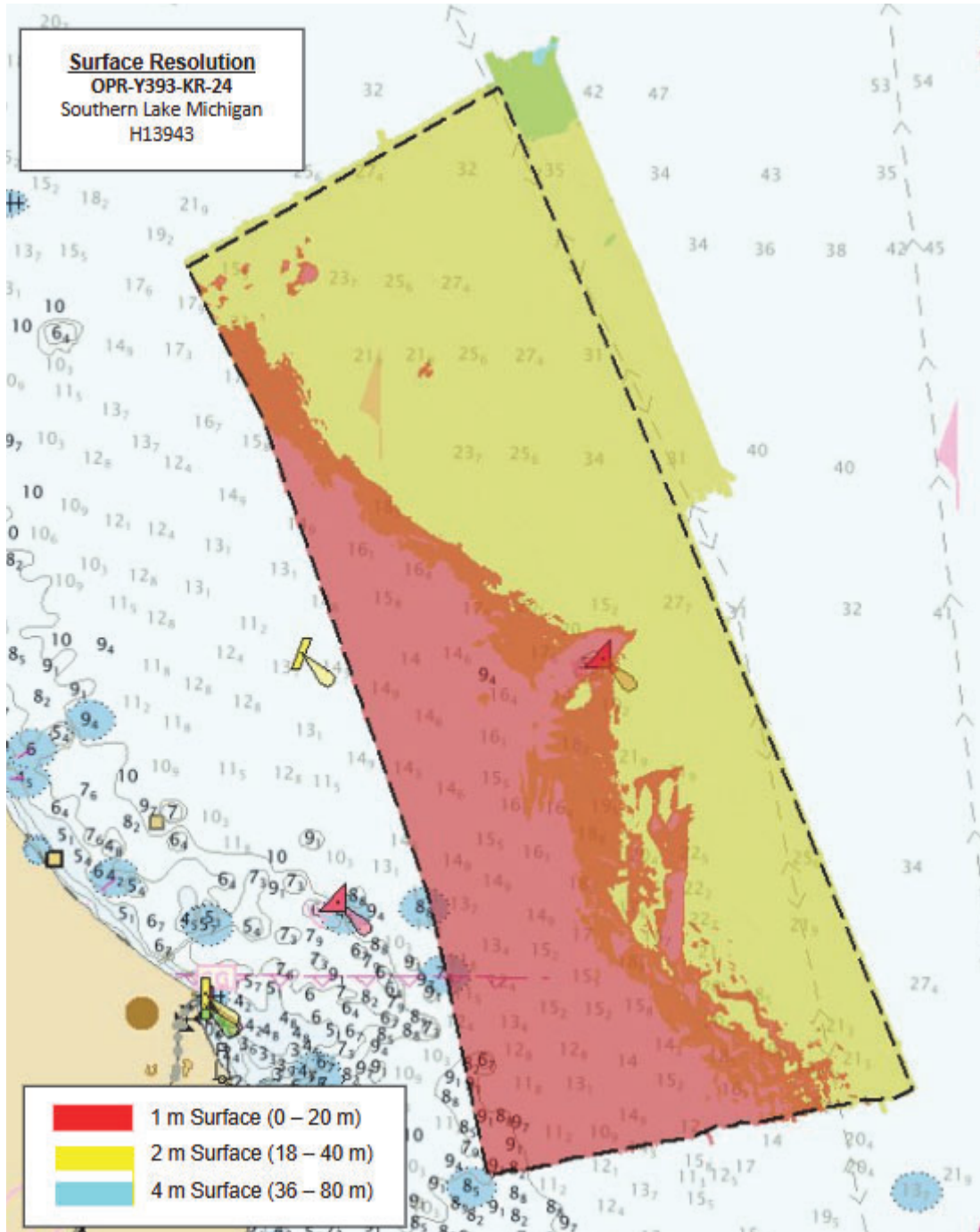
Figure 25: Image representing 1 m, 2 m, and 4 m finalized CUBE surface resolutions in H13943
