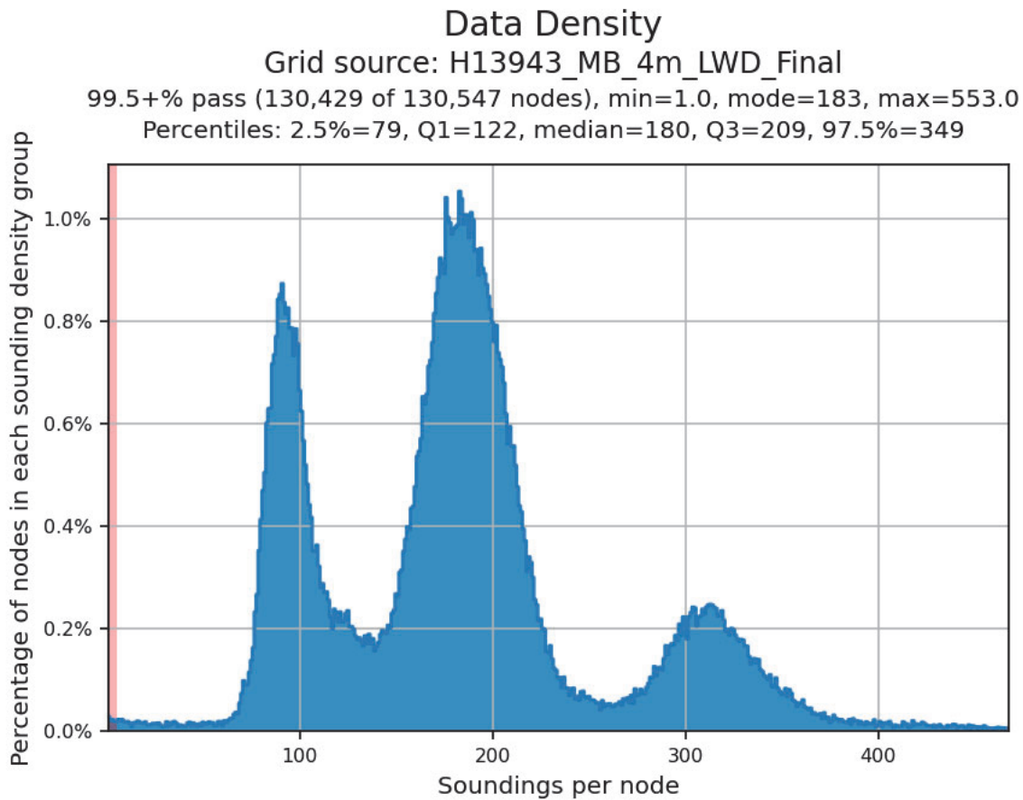
Figure 23: Finalized 4 m CUBE surface density statistics for H13943
