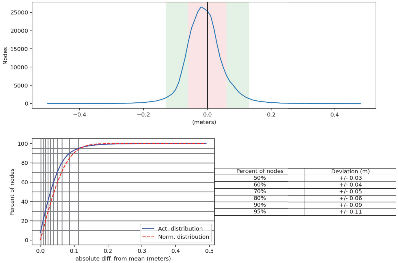
Figure 11: Junction analysis between H13943 and H13942 Finalized 2 m MBES CUBE surface
