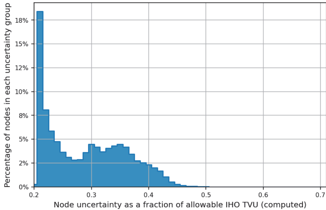
Figure 7: Finalized 2 m CUBE surface TVU statistics for H13943
