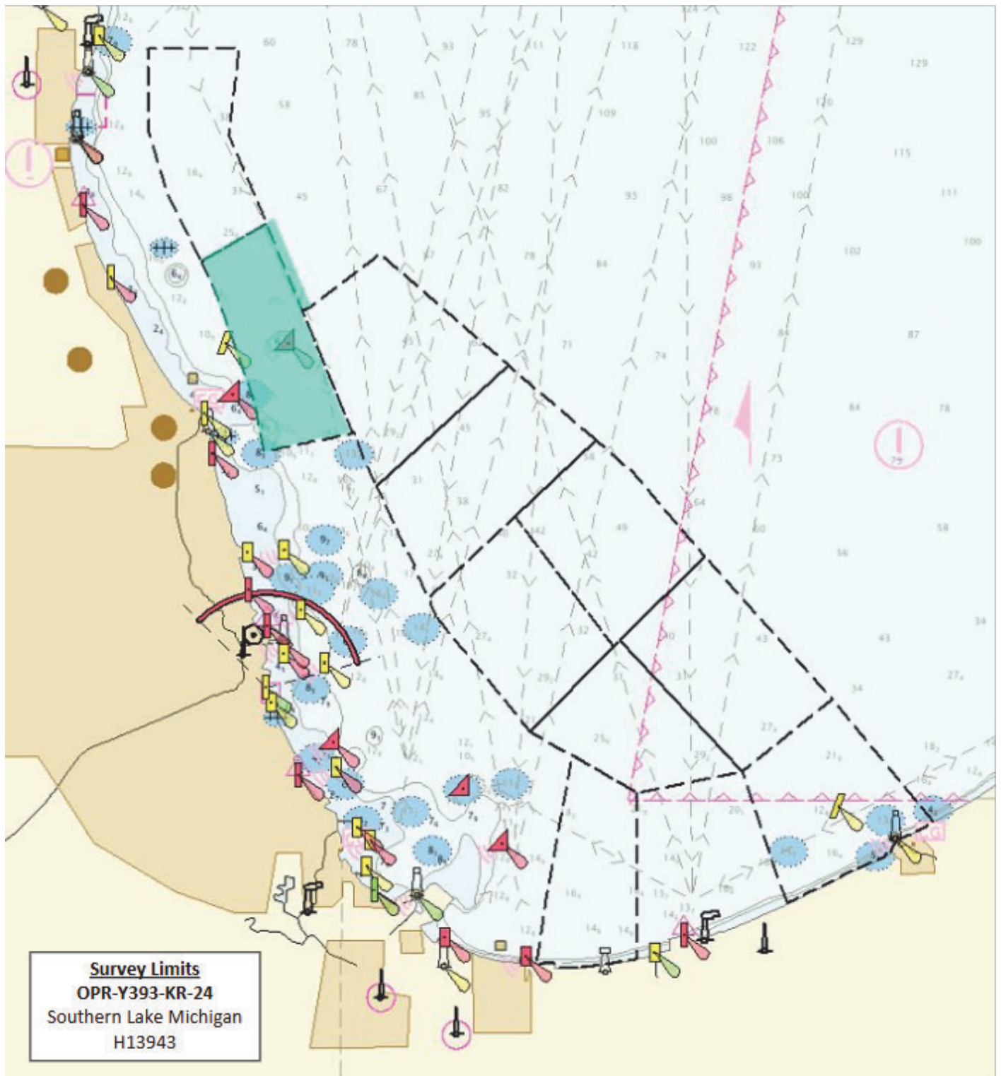
Figure 1: Overview of project survey limits (H13943 shown in blue), overlaid onto Chart US2MI01M
