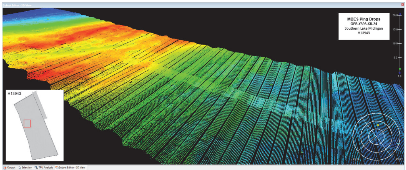
Figure 18: Example of MBES ping drops observed from R/V Benthos on 10/10/2024
