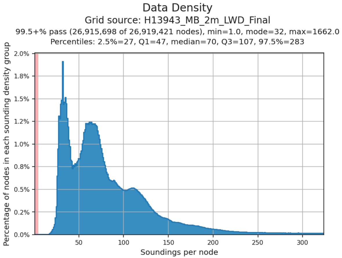
Figure 22: Finalized 2 m CUBE surface density statistics for H13943
