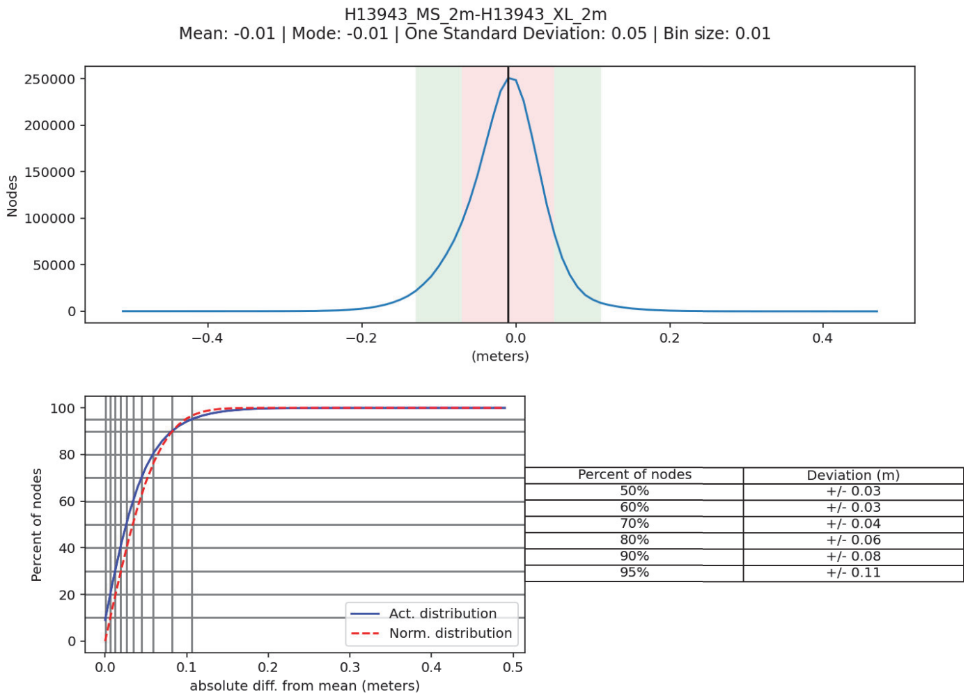
Figure 5: H13943 crossline to mainscheme difference statistics
