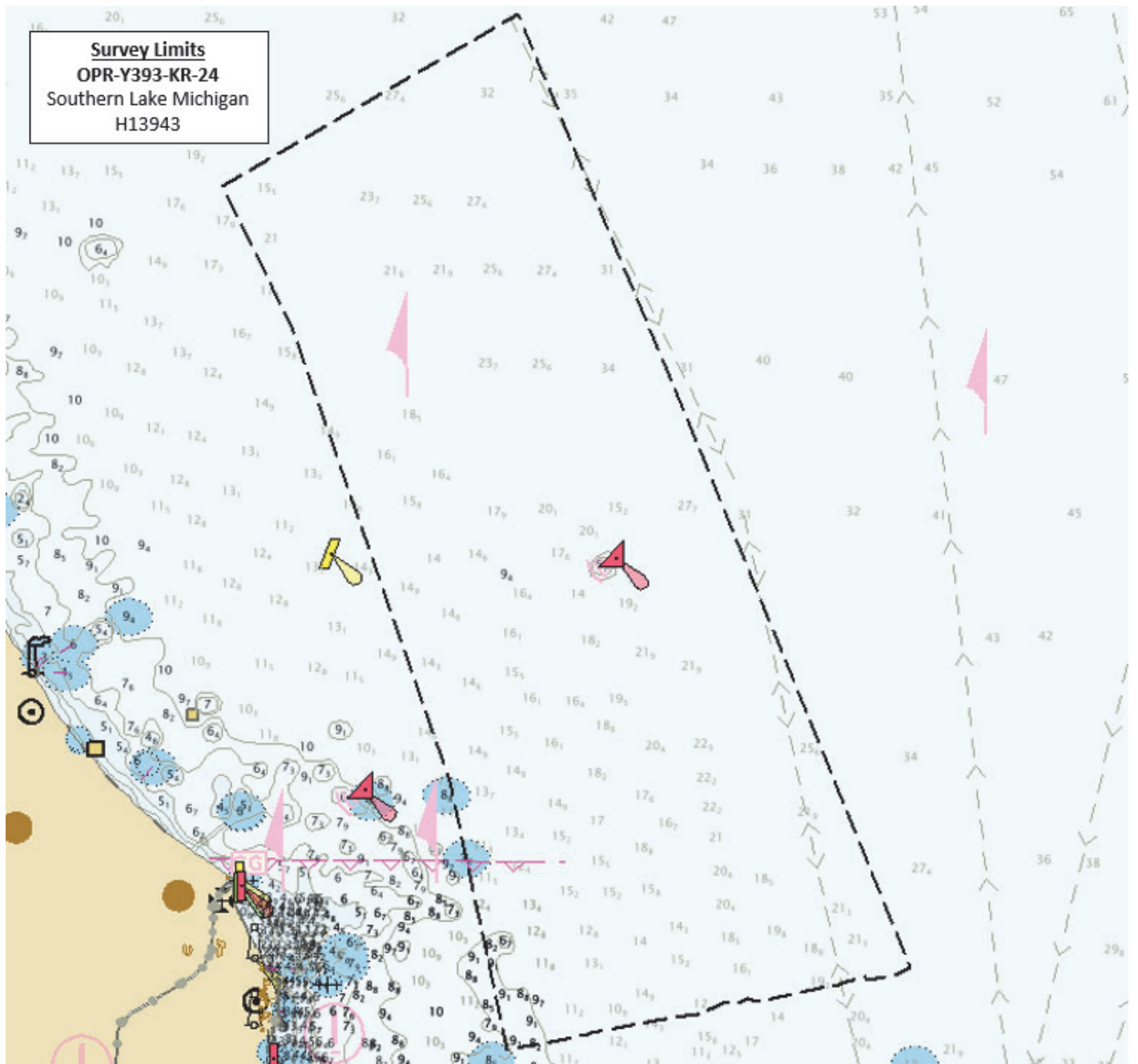
Figure 2: H13943 survey limits overlaid onto Charts US4IL1YX, US4IL1YY, and US5CHILL
