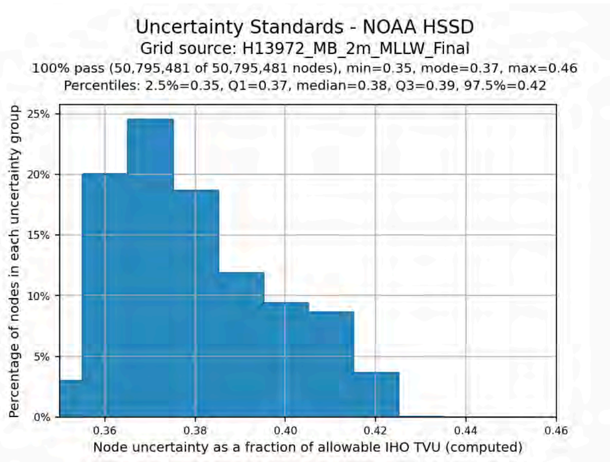
Figure 6: Node TVU Statistics - 2 meter, Finalized
