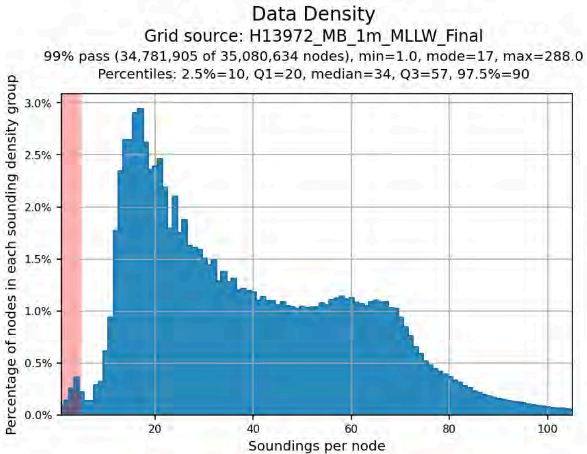
Figure 10: Node Density Statistics - 1 meter, Finalized
