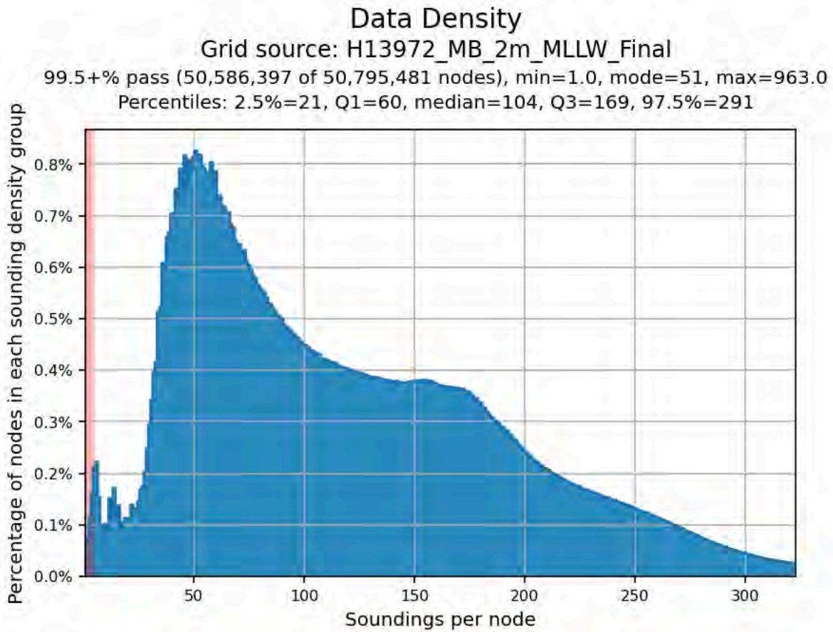
Figure 11: Node Density Statistics - 2 meter, Finalized
