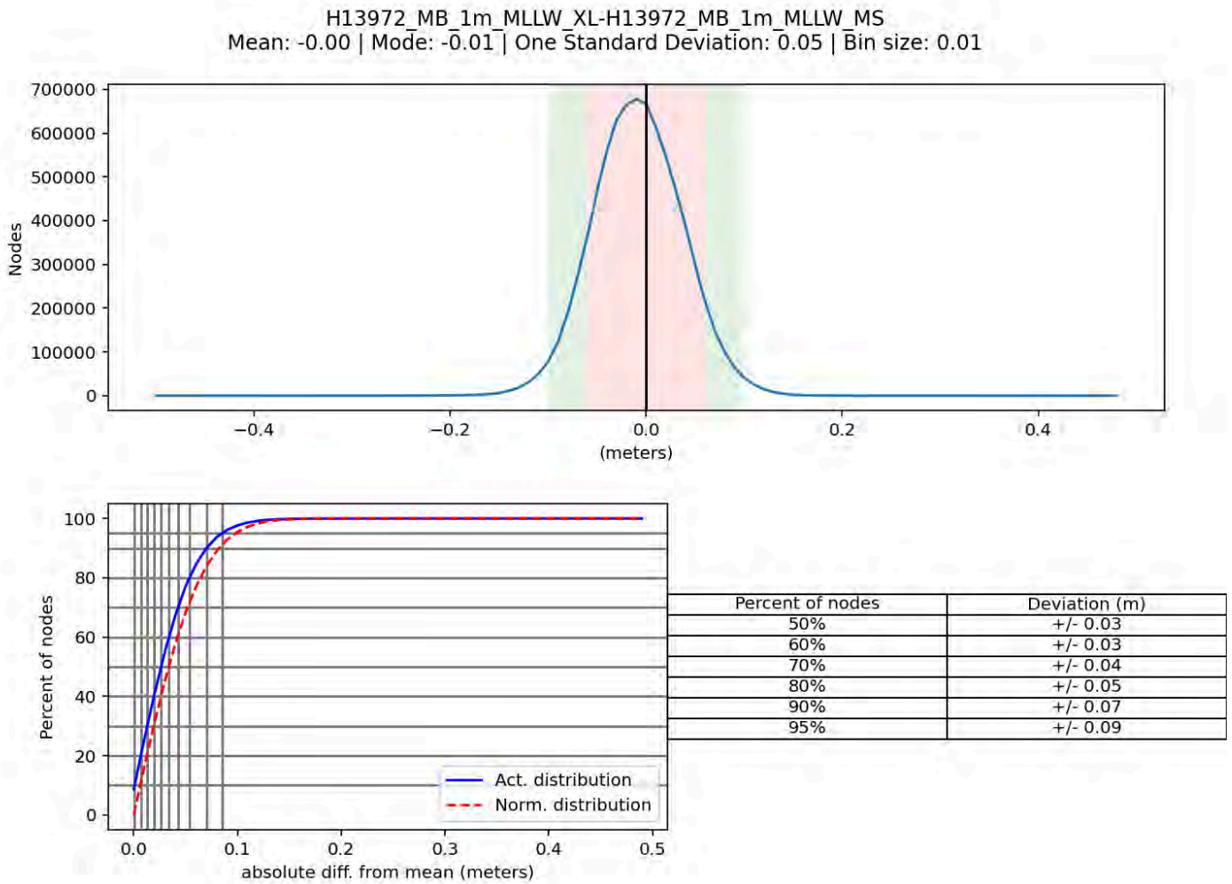
Figure 4: H13972 Crossline Difference
