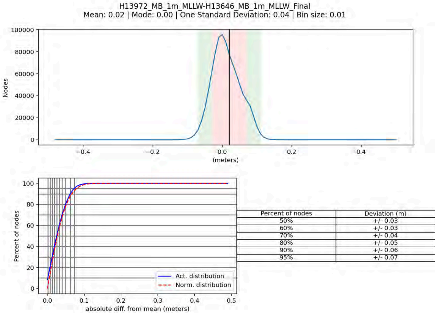
Figure 9: Distribution Summary Plot of Survey H13972 1-meter vs. H13646 1-meter
