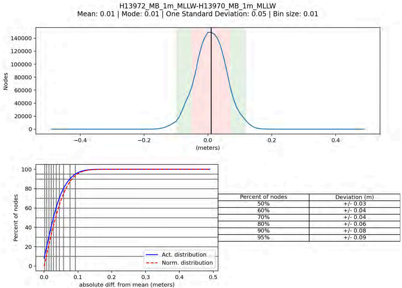
Figure 8: Distribution Summary Plot of Survey H13972 1-meter vs. H13970 1-meter
