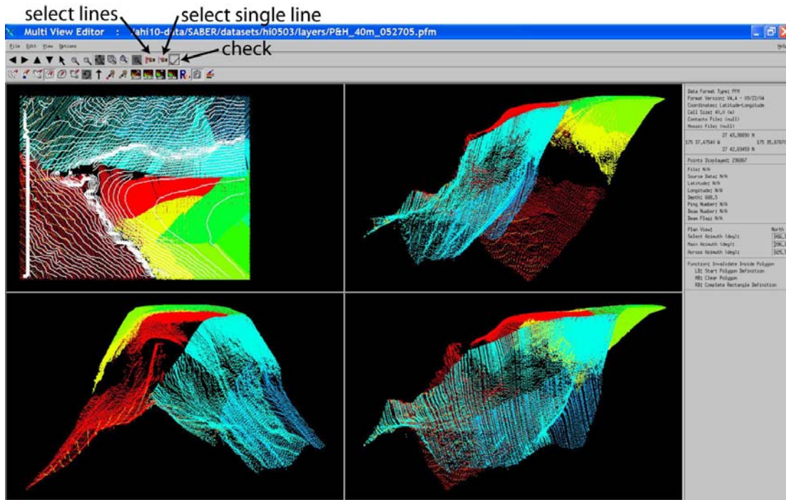
Figure PFM Edit: Several multibeam swaths, represented by different colors, are viewed simultaneously in the PFM editor and the grid can be edited viewing only any combination of files at the same time.
