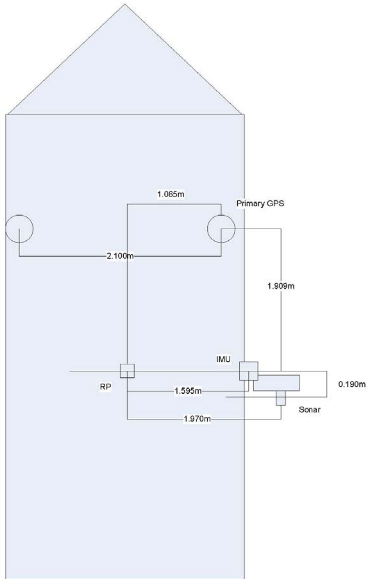
Plan View of NPS Osprey Sensor Layout
