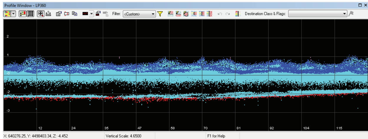
Figure 3 LP360 profile of shoal points on sand waves included in water column class (light blue), which ends up being excluded from the bare earth model. The surrounding classified bathymetry (red points) demonstrate how the bottom tracking algorithm only classifies the bottom edge of the ground/bathy points. This image also demonstrates the noise in the water column, extending down from the water's surface. Block 124.
