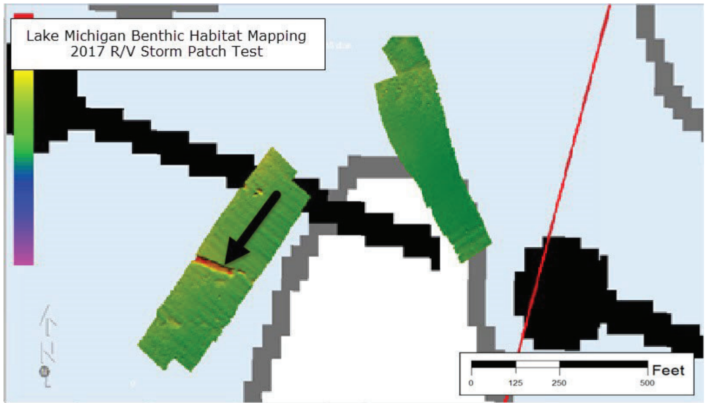
Figure 3. Patch test conducted over the Manitowoc Waterworks plant pipeline. Notice the structure was detected nearly 200 feet to the south of the charted position of the pipeline.
