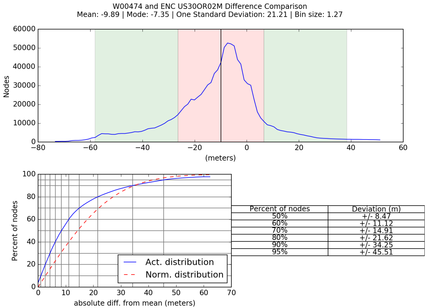
Figure 6: Difference surface statistics between W00474 and interpolated TIN surface from ENC US30OR02M
