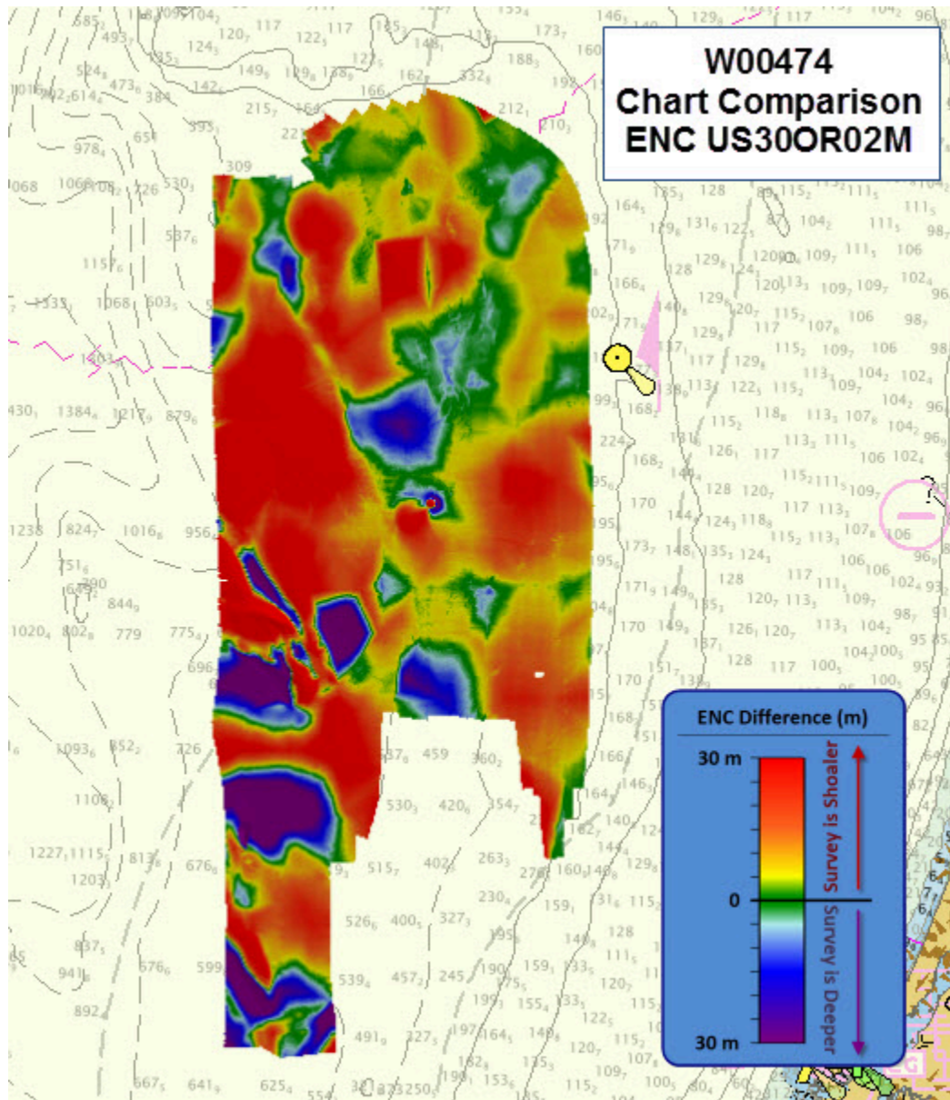
Figure 5: Difference surface between W00474 and interpolated TIN surfaces from ENC US30OR2M
