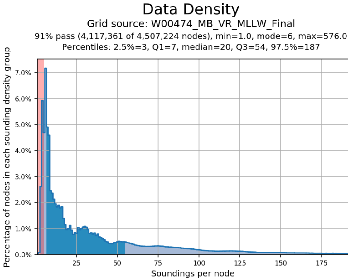
Figure 3: W00474 compliance with density requirements
