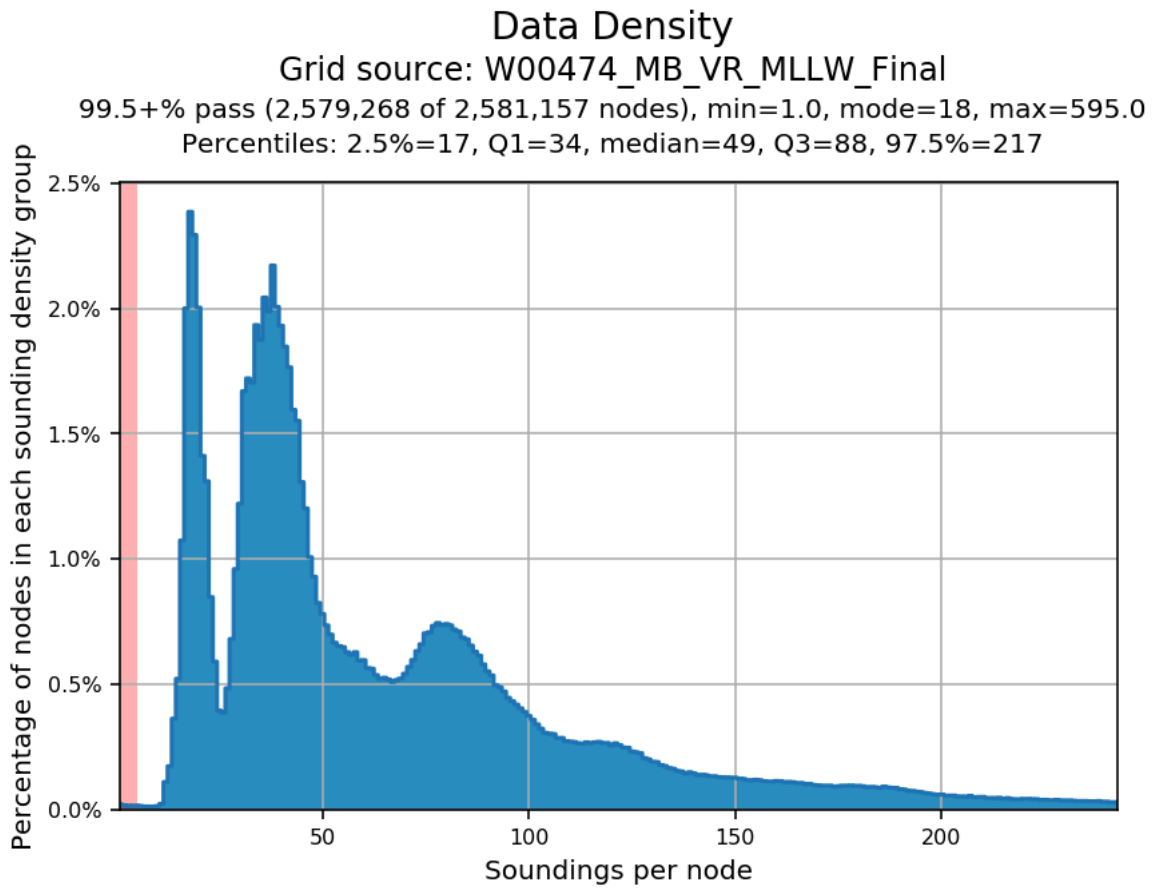
Figure 4: Density compliance run during office review.
