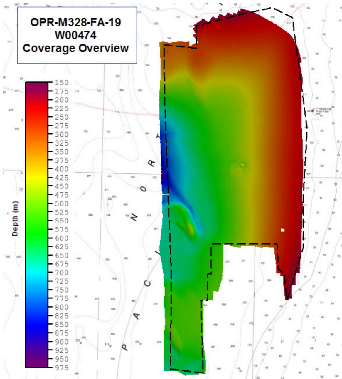
Figure 1: W00474 Coverage overview with sheet limits shown in black
