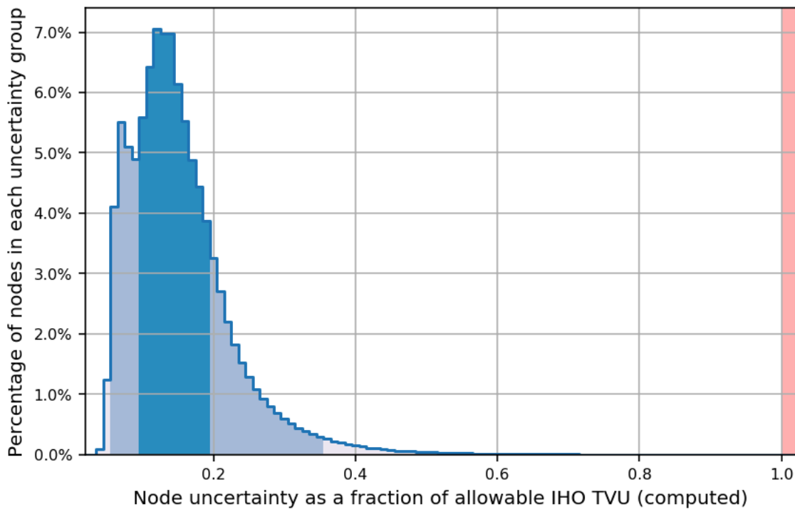
Figure 2: W00474 compliance with uncertainty standards
