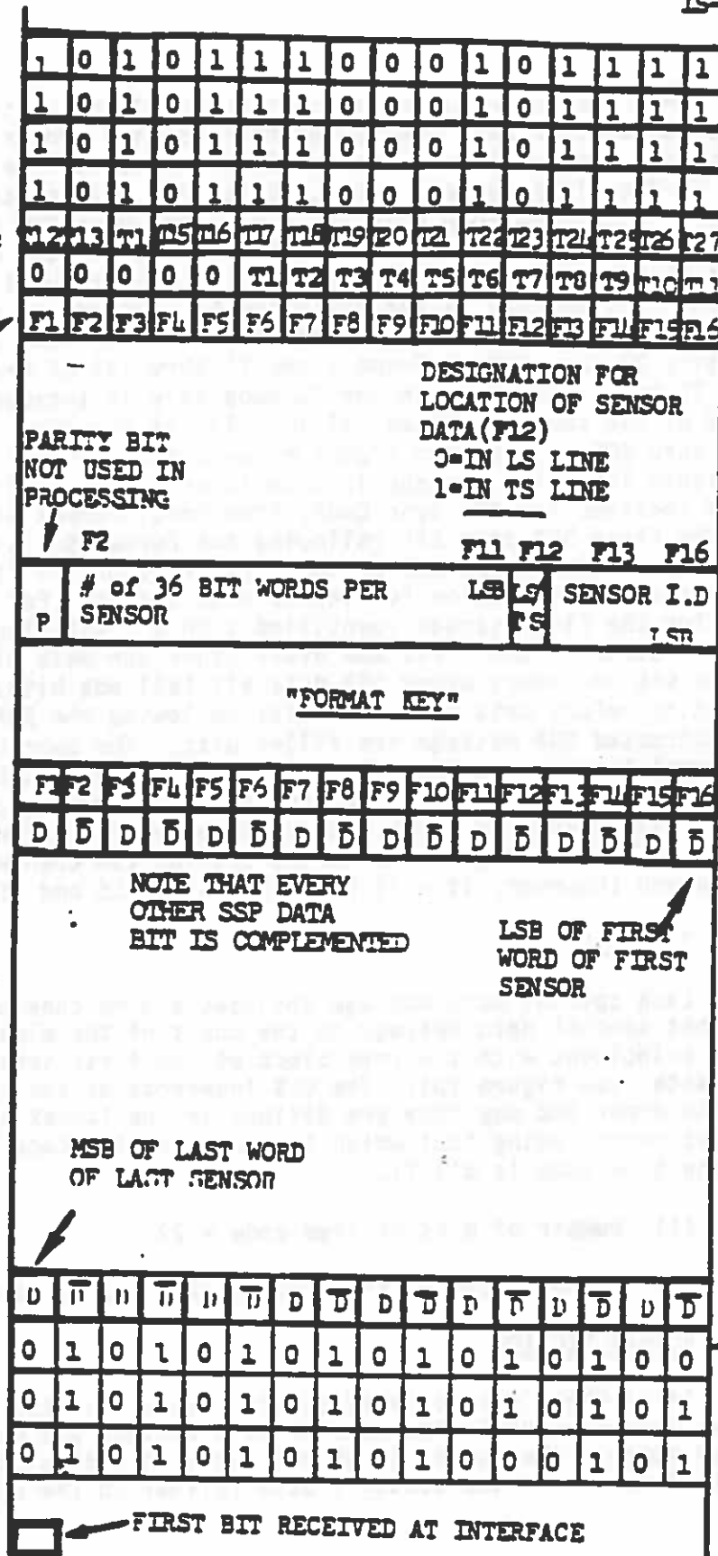
FIGURE 13: SSP MESSAGE FORMAT
