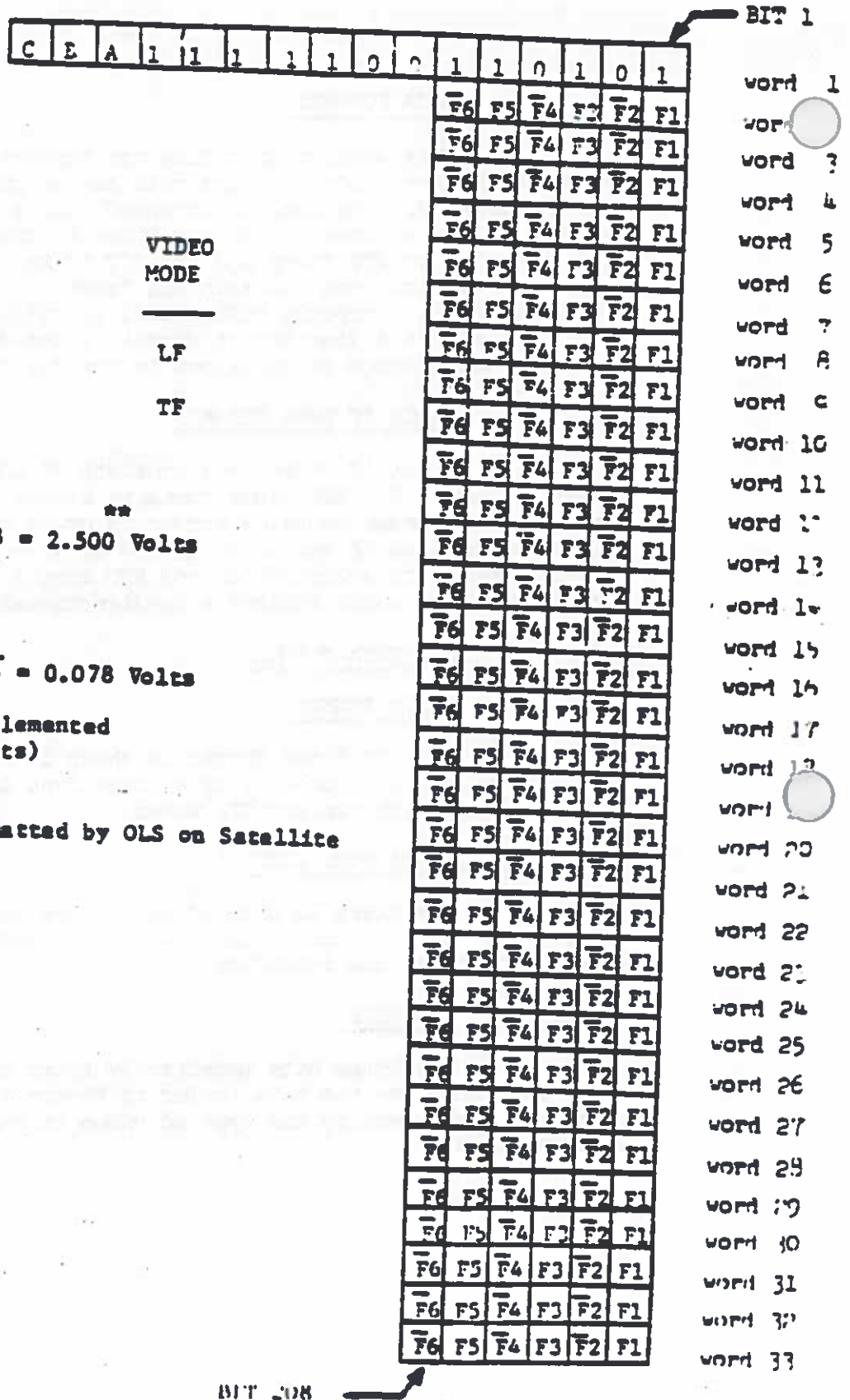
FIGURE 4: SDF FRAME FORMAT
