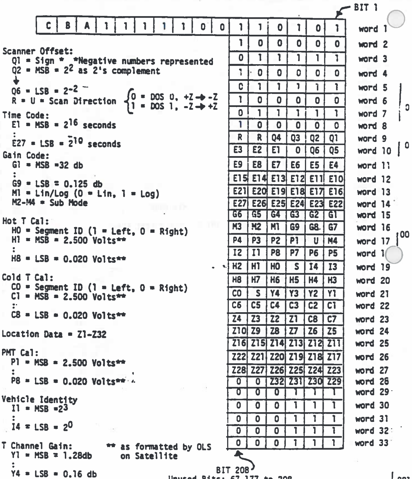
FIGURE 9: SDF SUB-SYNC FRAME FORMAT
