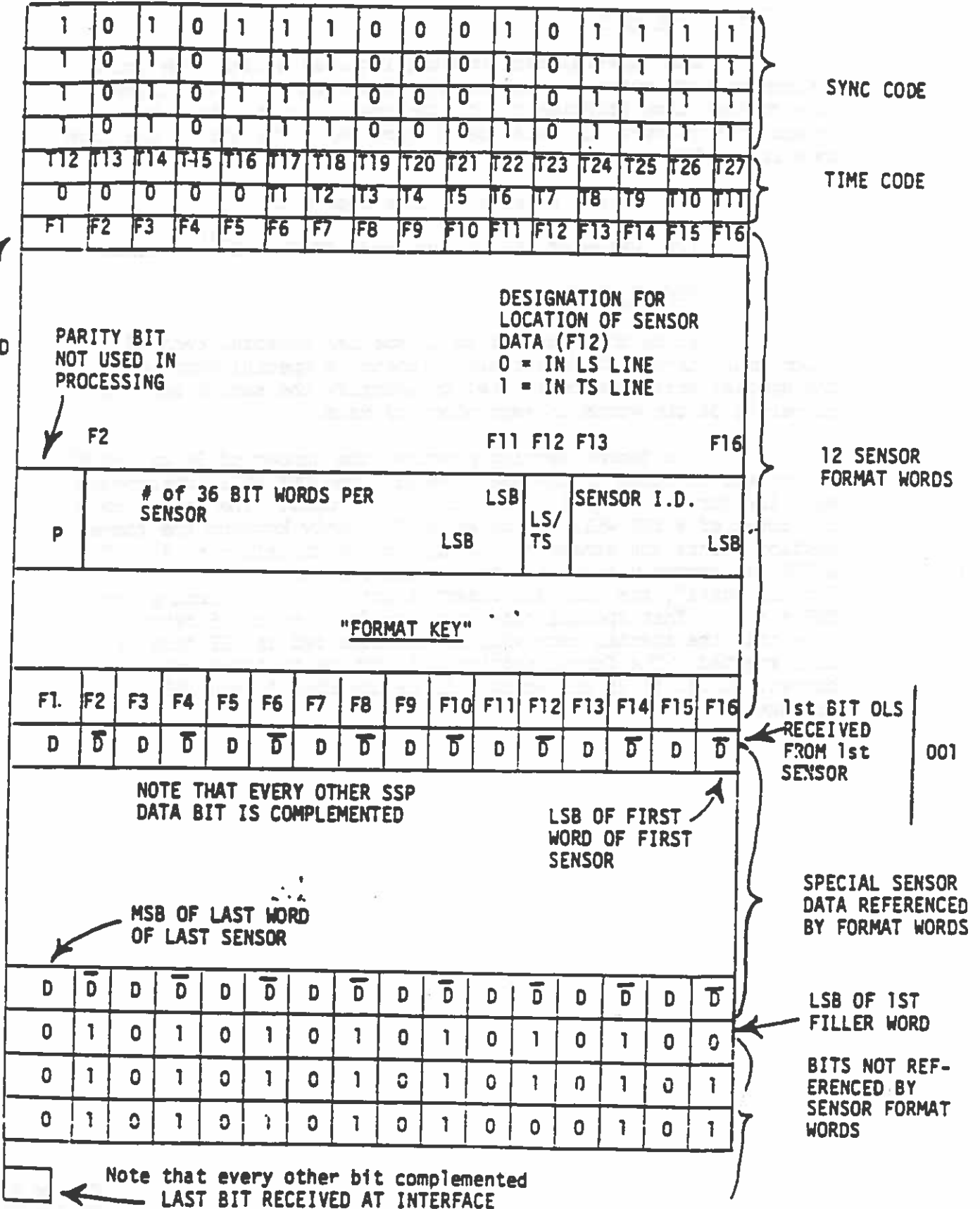
FIGURE 30: SSP MESSAGE FORMAT
