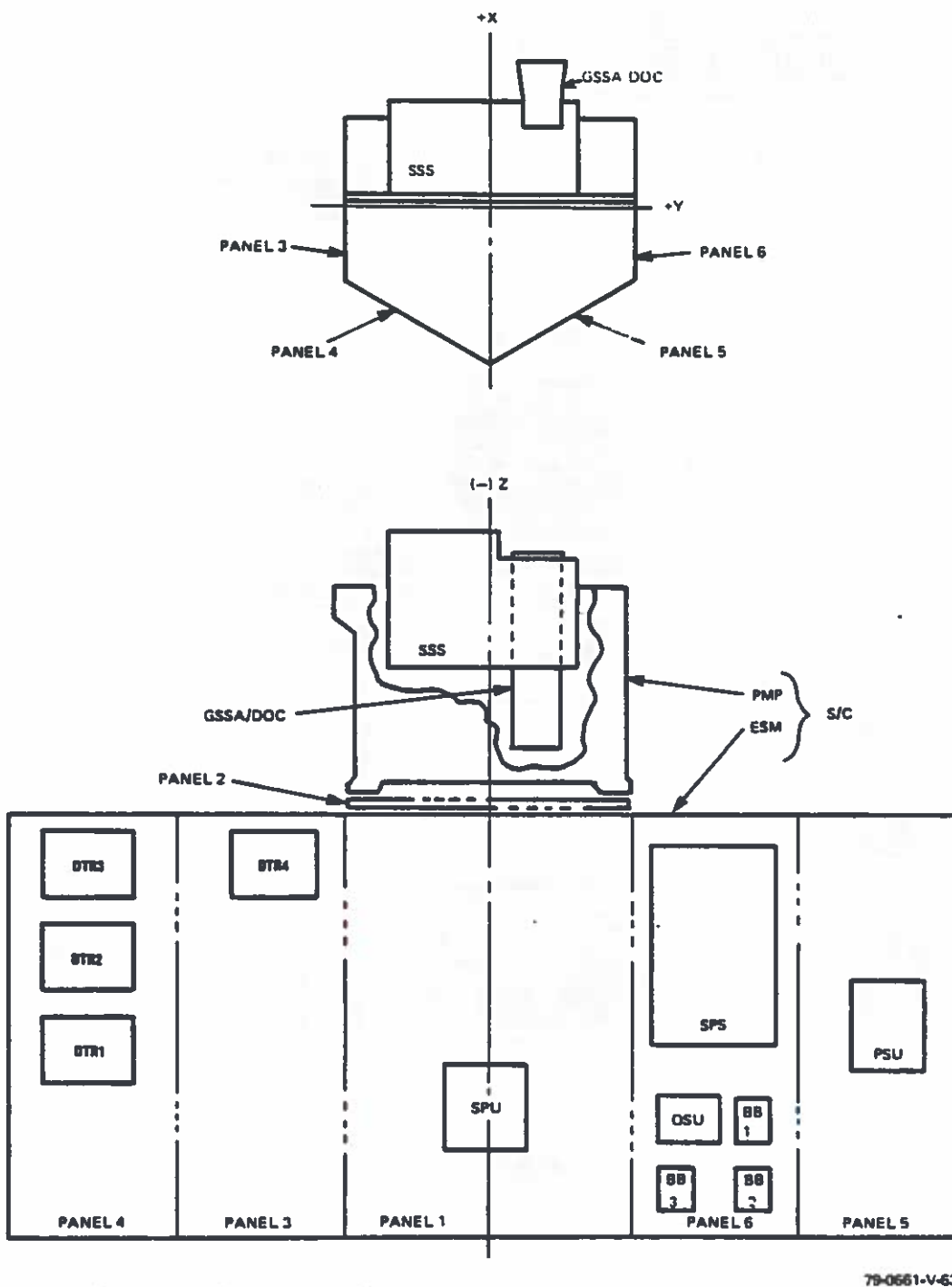
Figure 2.2.0-3. Spacecraft Placement of OLS Assemblies
