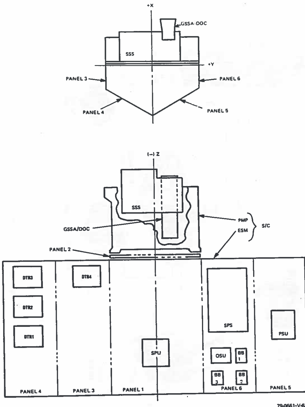
Figure 2.2.0-3. Spacecraft Placement of OLS Assemblies (S11 - S14)
