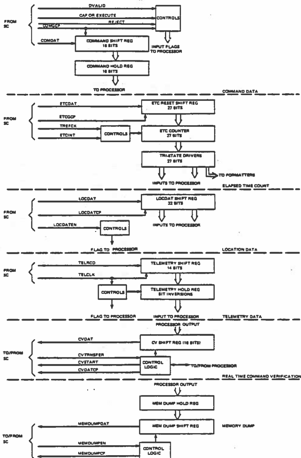
Figure 2.1.3.2-3. Spacecraft Interfaces
